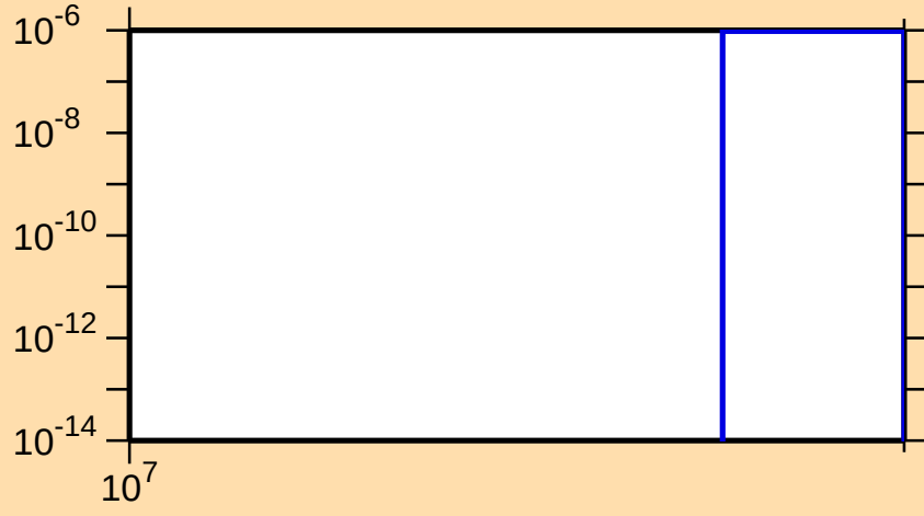
\sigma vs. E for ^{52}\text{Sc}(n,2np)
