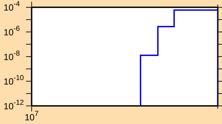
\sigma vs. E for ^{52}\text{Sc}(n,nt)
