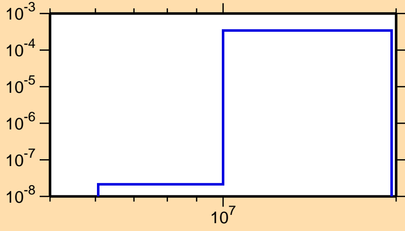
\sigma vs. E for ^{52}\text{Sc}(n,t)
