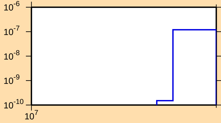
\sigma vs. E for ^{72}\text{Se}(\text{mt } 45)
