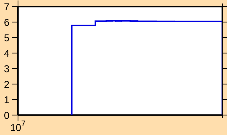
\Delta\sigma/\sigma vs. E for ^{72}\text{Se}(n,\text{nonel.})
