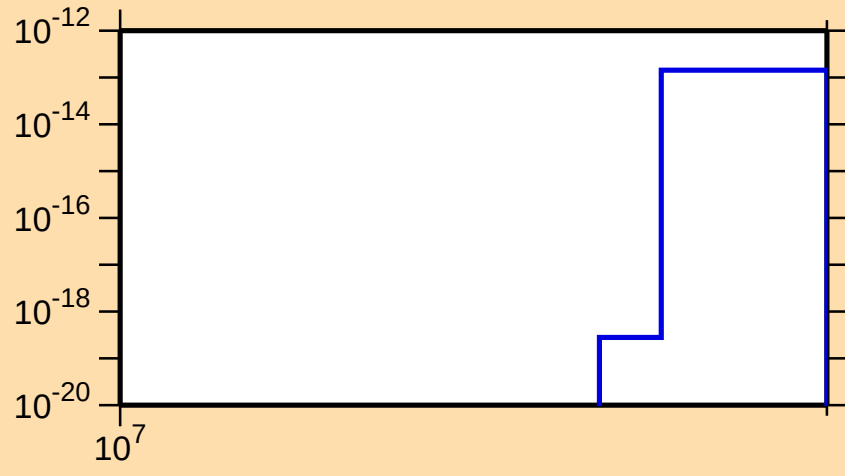
\sigma vs. E for ^{72}\text{Se}(\text{mt } 34)
