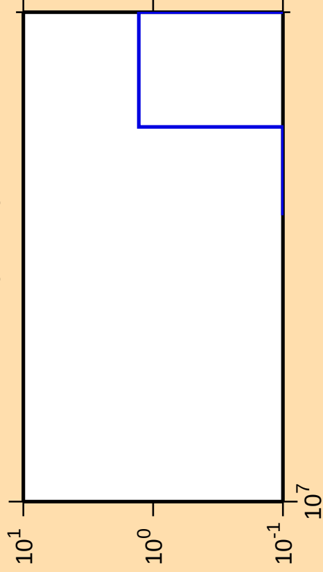
\Delta\sigma/\sigma vs. E for ^{72}\text{Se}(\text{mt } 34)
