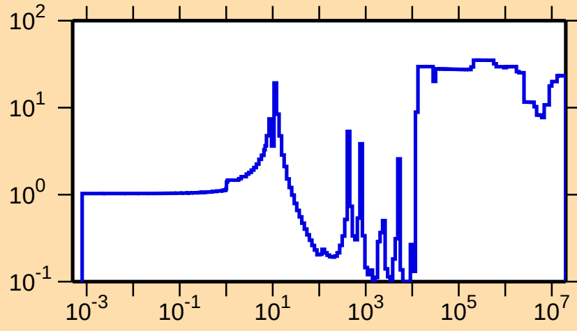
\Delta\sigma/\sigma vs. E for ^{72}\text{Se}(n,\text{el.})
