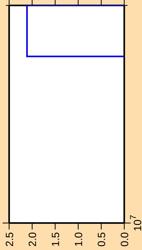
\Delta\sigma/\sigma vs. E for ^{72}\text{Se}(n,2np)
