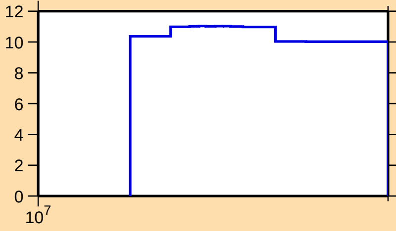
\Delta\sigma/\sigma vs. E for ^{72}\text{Se}(n,\text{tot.})
