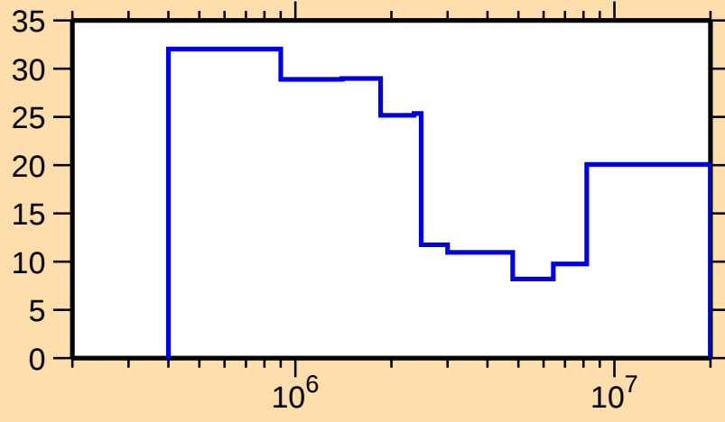
\Delta\sigma/\sigma vs. E for ^{72}\text{Se}(\text{n,el.})
