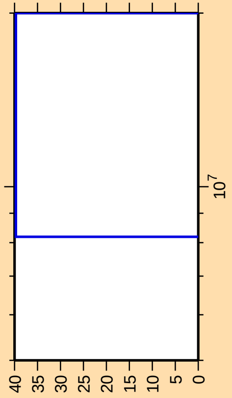
\Delta\sigma/\sigma vs. E for ^{72}\text{Se}(n,p)
