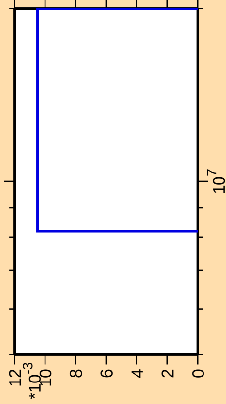
\Delta\sigma/\sigma vs. E for ^{72}\text{Se}(\text{mt } 34)
