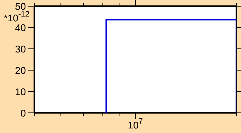
\sigma vs. E for ^{72}\text{Se}(n,\text{nd})
