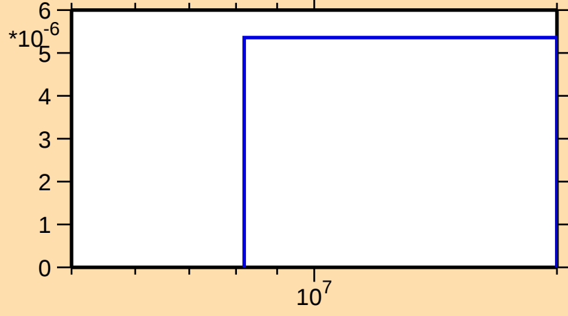
\sigma vs. E for ^{72}\text{Se}(n,\text{pd})
