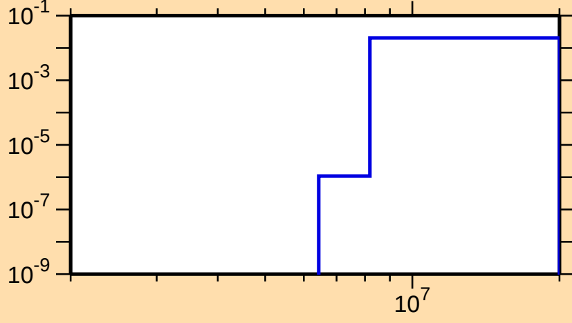
\sigma vs. E for ^{72}\text{Se}(n,n\alpha)
