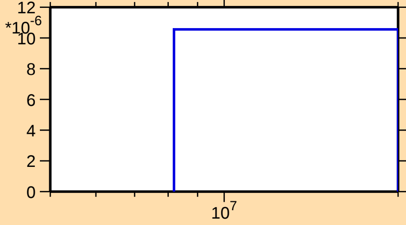
\sigma vs. E for ^{72}\text{Se}(n,t)
