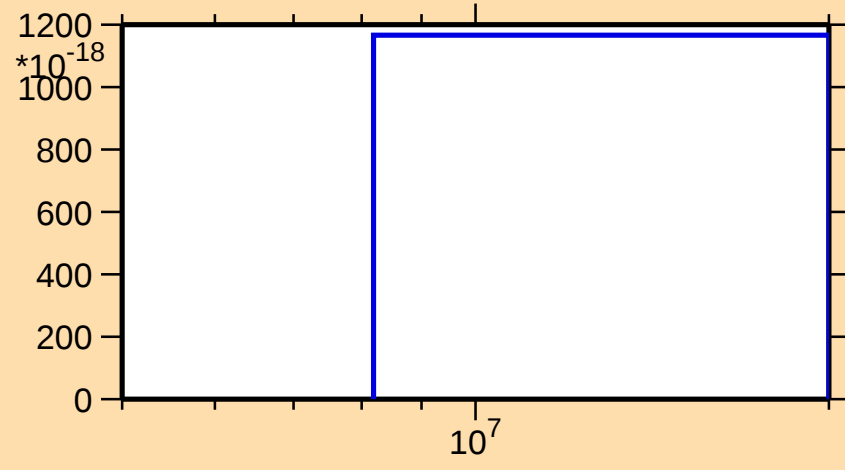
\sigma vs. E for ^{72}\text{Se}(\text{mt } 34)
