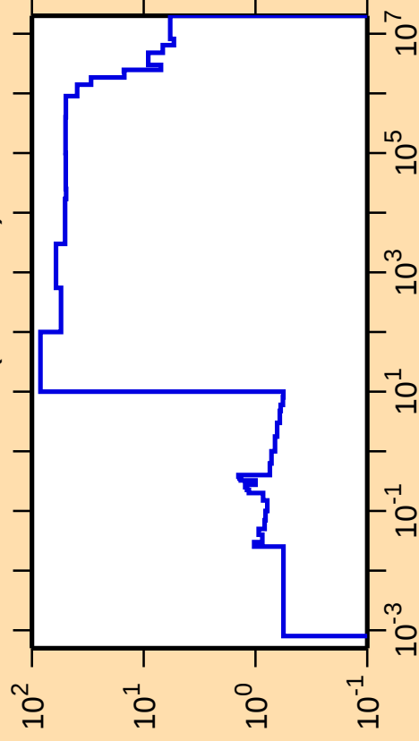
\Delta\sigma/\sigma vs. E for ^{72}\text{Se}(n,\text{nonel.})
