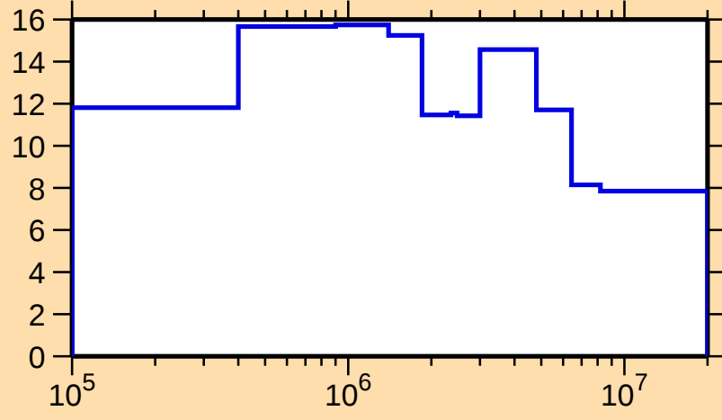
\Delta\sigma/\sigma vs. E for ^{83}\text{Se}(\text{n,el.})
