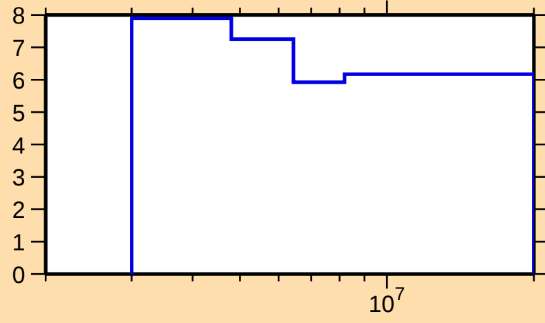
\Delta\sigma/\sigma vs. E for ^{83}\text{Se}(n,n\text{onrel.})
