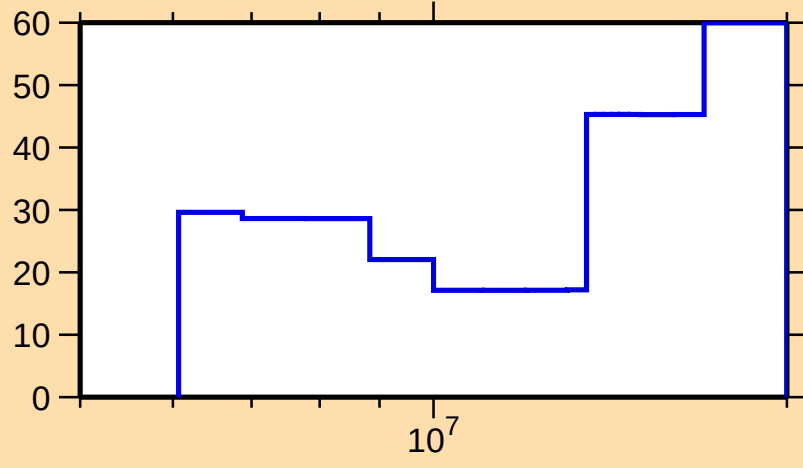
\Delta\sigma/\sigma vs. E for ^{86}\text{Se}(n,2n)
