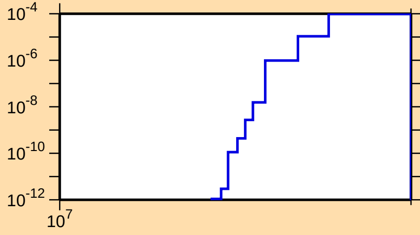
\sigma vs. E for ^{86}\text{Se}(n,d)
