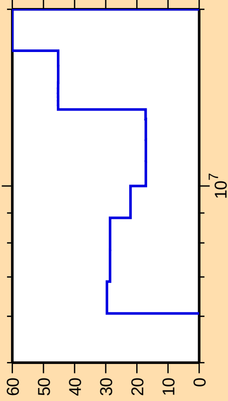
\Delta\sigma/\sigma vs. E for ^{86}\text{Se}(n,2n)
