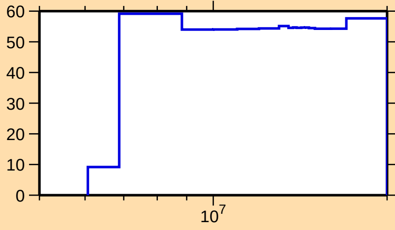
\Delta\sigma/\sigma vs. E for ^{86}\text{Se}(n,\text{inel.})
