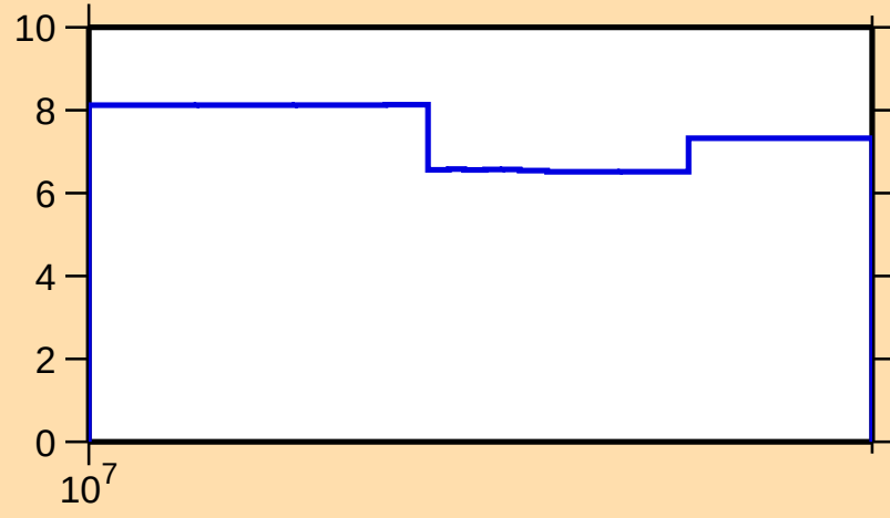
\Delta\sigma/\sigma vs. E for ^{86}\text{Se}(n,\text{nonel.})
