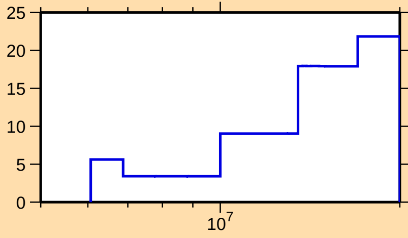
\Delta\sigma/\sigma vs. E for ^{86}\text{Se}(n,\text{tot.})
