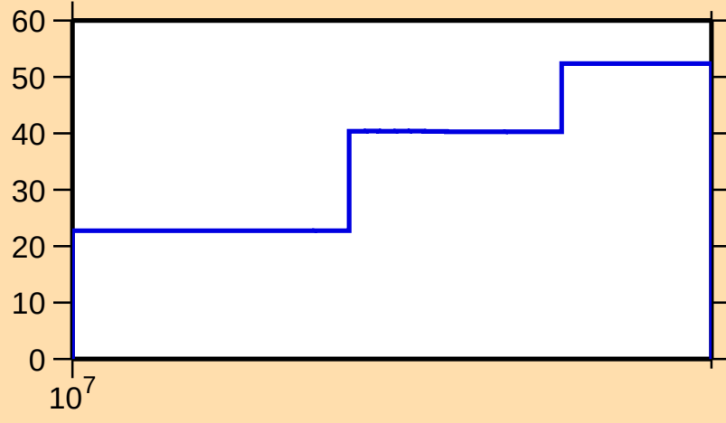
\Delta\sigma/\sigma vs. E for ^{86}\text{Se}(n,\text{el.})
