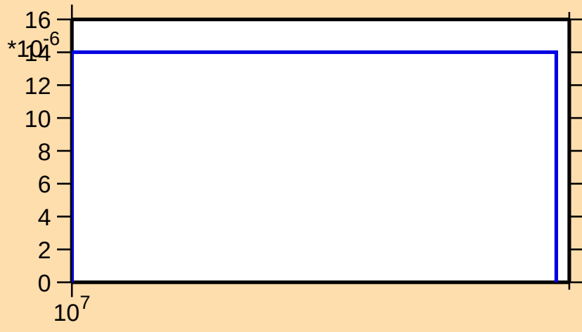
\sigma vs. E for ^{86}\text{Se}(n,p)
