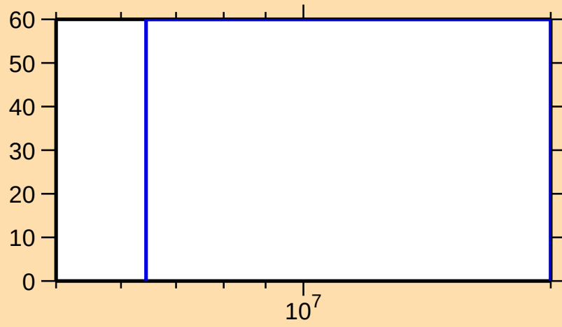
\Delta\sigma/\sigma vs. E for ^{86}\text{Se}(n,n\text{cont.})
