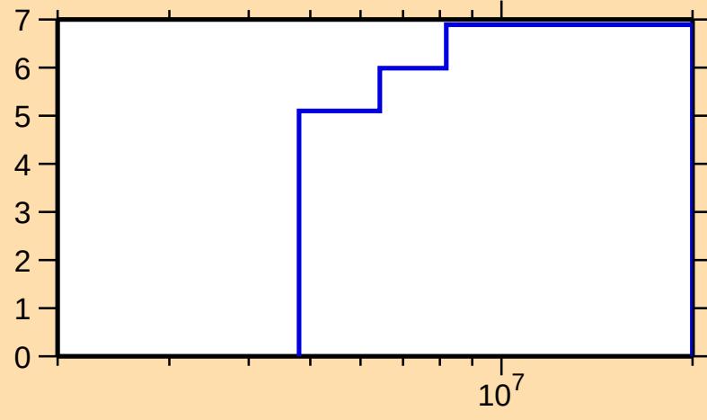
\Delta\sigma/\sigma vs. E for ^{86}\text{Se}(n,\text{nonel.})
