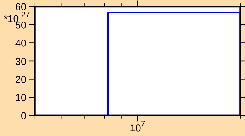
\sigma vs. E for ^{86}\text{Se}(n,\text{He}3)
