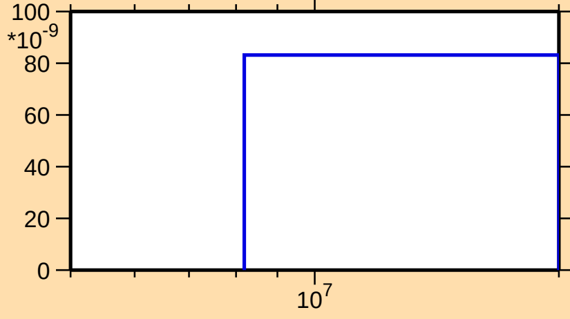
\sigma vs. E for ^{86}\text{Se}(n,np)
