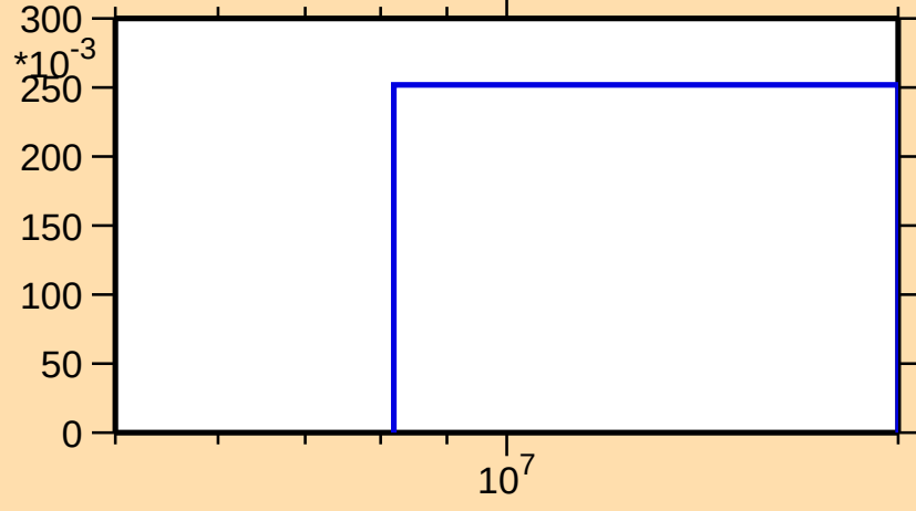
\sigma vs. E for ^{86}\text{Se}(n,3n)
