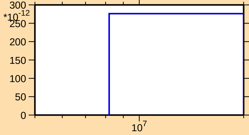
\sigma vs. E for ^{86}\text{Se}(n,nt)
