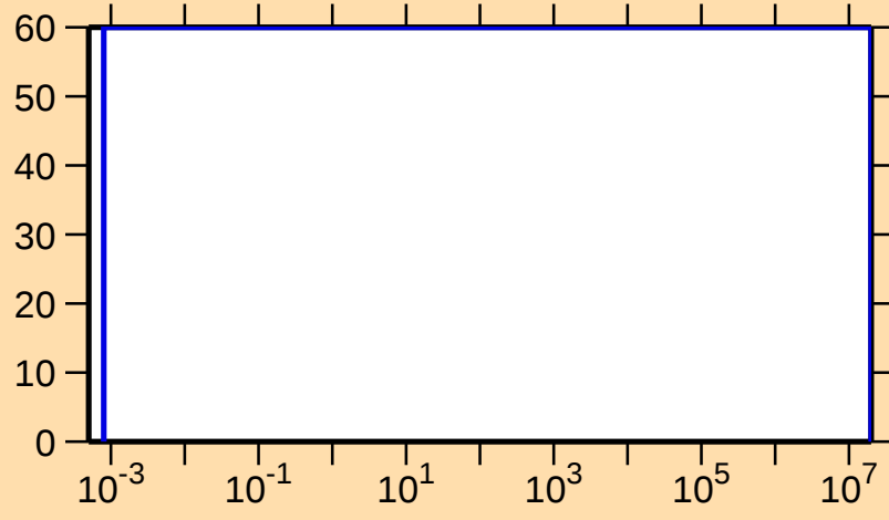
\Delta\sigma/\sigma vs. E for ^{265}\gamma )
