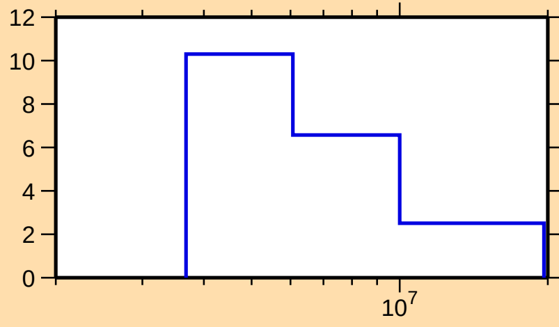
\Delta\sigma/\sigma vs. E for ^{26}\text{Si}(n,\text{tot.})
