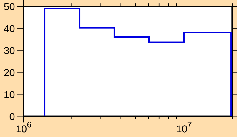
\Delta\sigma/\sigma vs. E for ^{26}\text{Si}(n,\text{inel.})
