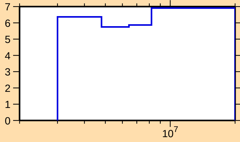
\Delta\sigma/\sigma vs. E for ^{26}\text{Si}(n,n\text{onel.})
