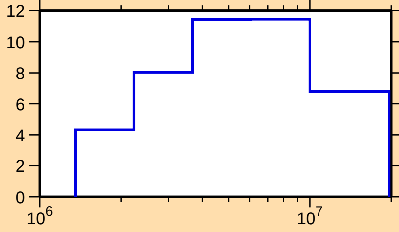
\Delta\sigma/\sigma vs. E for ^{28}\text{Si}(\text{n,el.})
