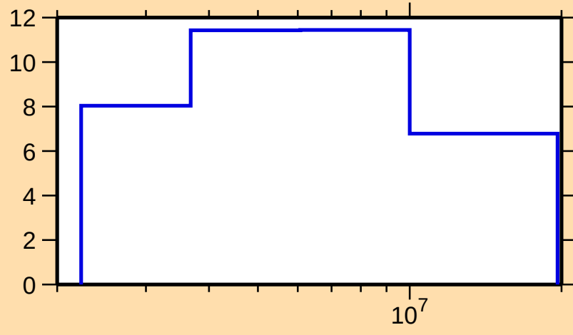
\Delta\sigma/\sigma vs. E for ^{28}\text{Si}(n,\text{el.})
