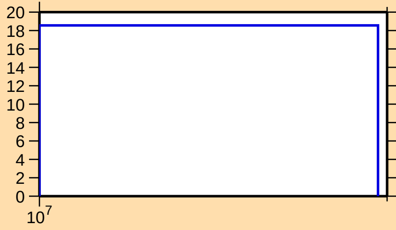
\Delta\sigma/\sigma vs. E for ^{28}\text{Si}(\text{n},\text{inel.})
