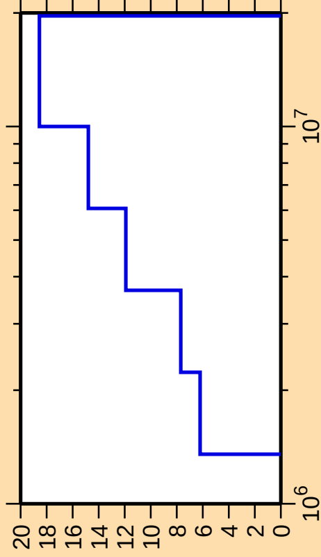
\Delta\sigma/\sigma vs. E for ^{28}\text{Si}(\text{n,inel.})
