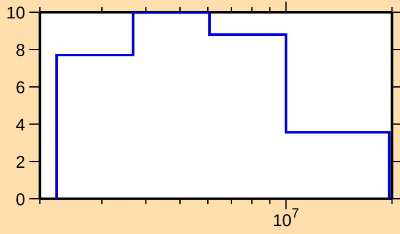
\Delta\sigma/\sigma vs. E for ^{28}\text{Si}(n,\text{tot.})
