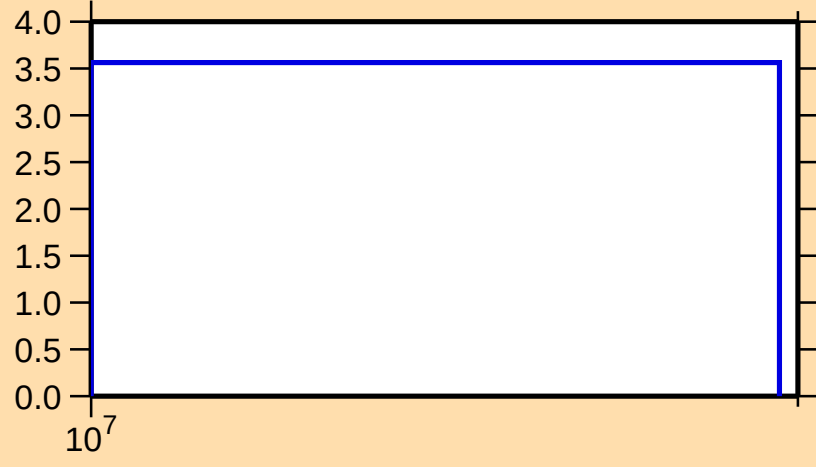
\Delta\sigma/\sigma vs. E for ^{28}\text{Si}(\text{n},\text{tot.})
