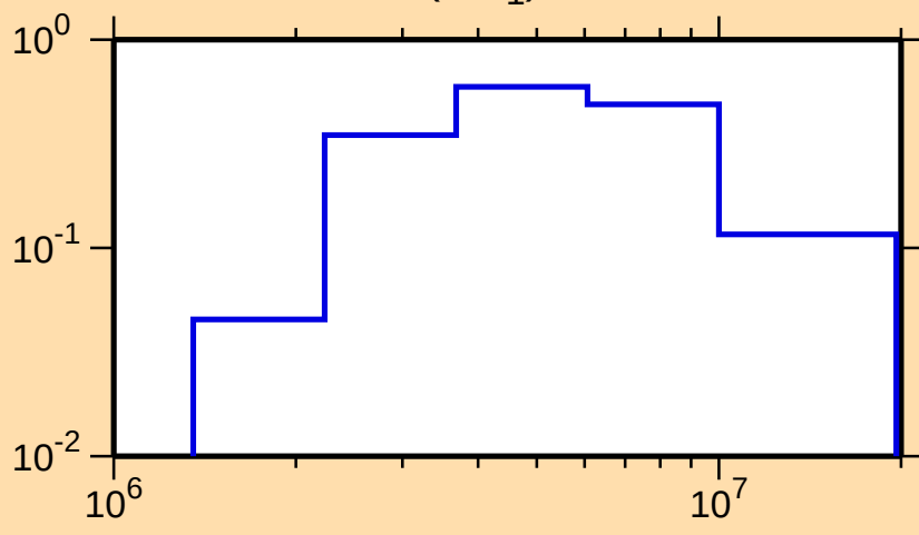
\sigma vs. E for ^{28}\text{Si}(n,n_1)
