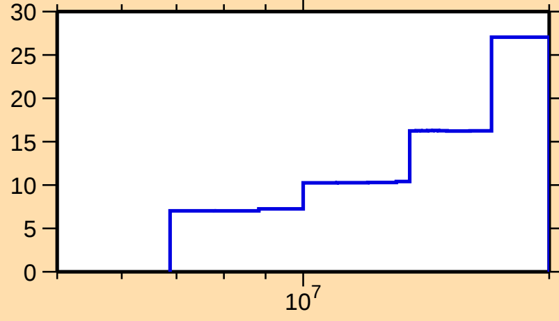
\Delta\sigma/\sigma vs. E for ^{29}\text{Si}(\text{n},\text{inel.})
