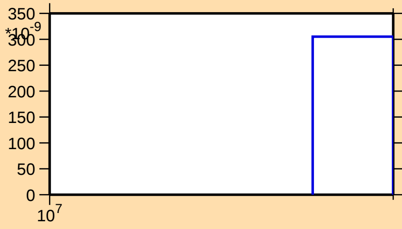
\sigma vs. E for ^{29}\text{Si}(n,\text{nd})
