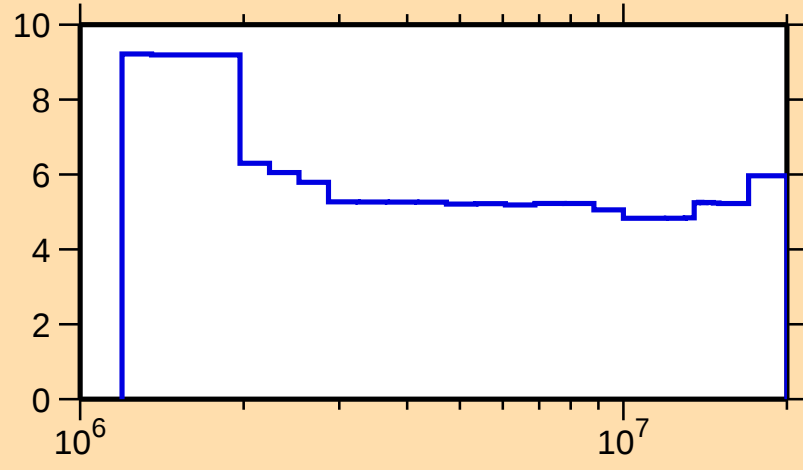
\Delta\sigma/\sigma vs. E for ^{29}\text{Si}(n,\text{nonel.})
