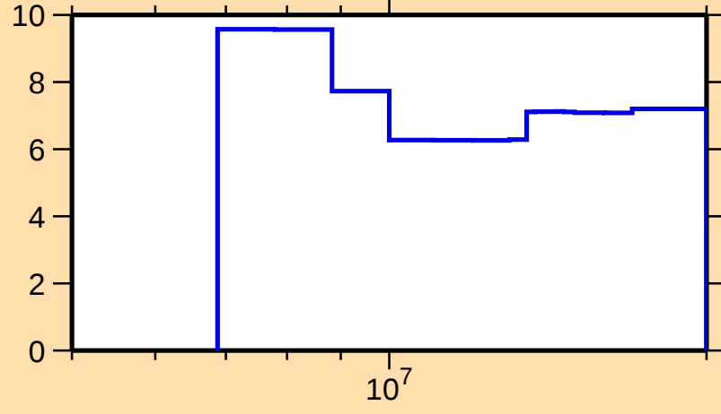
\Delta\sigma/\sigma vs. E for ^{29}\text{Si}(\text{n},\text{el.})
