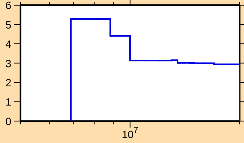
\Delta\sigma/\sigma vs. E for ^{29}\text{Si}(\text{n},\text{tot.})
