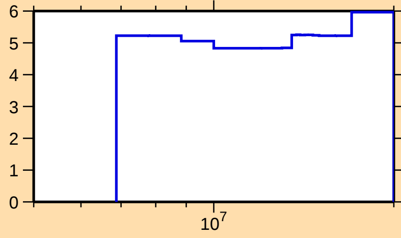
\Delta\sigma/\sigma vs. E for ^{29}\text{Si}(\text{n},\text{nonel.})
