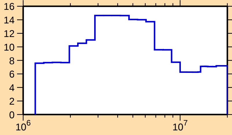
\Delta\sigma/\sigma vs. E for ^{29}\text{Si}(\text{n,el.})
