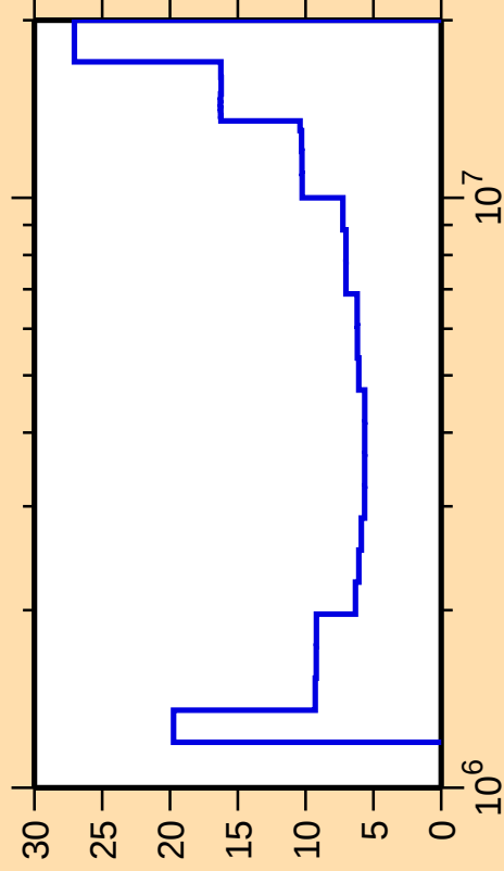
\Delta\sigma/\sigma vs. E for ^{29}\text{Si}(\text{n,inel.})
