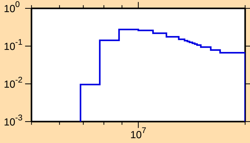
\sigma vs. E for ^{29}\text{Si}(n,n\text{cont.})
