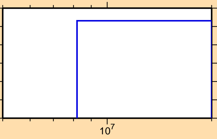
\sigma vs. E for ^{33}\text{Si}(n,d)
