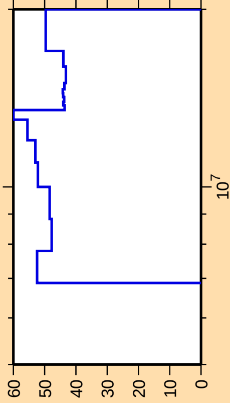
\Delta\sigma/\sigma vs. E for ^{34}\text{Si}(n,\text{ncont.})
