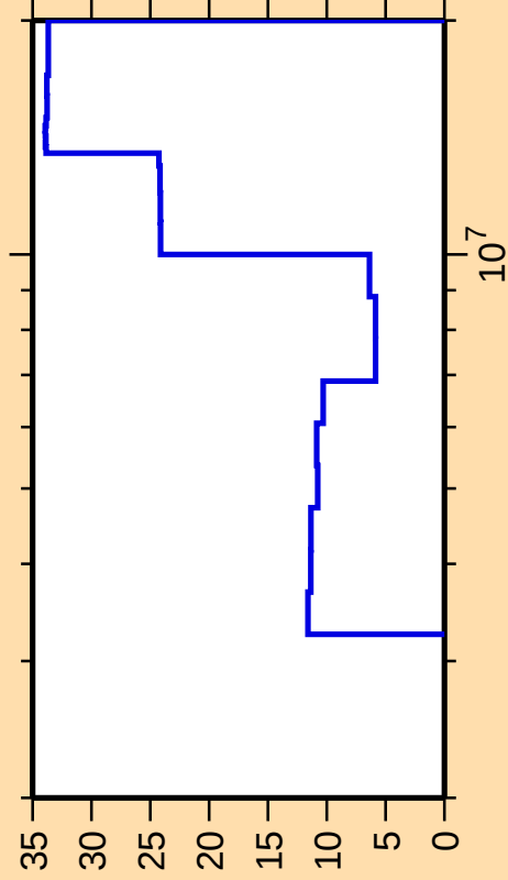
\Delta\sigma/\sigma vs. E for ^{34}\text{Si}(\text{n,inel.})
