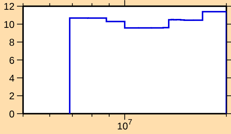
\Delta\sigma/\sigma vs. E for ^{34}\text{Si}(n,\text{nonel.})
