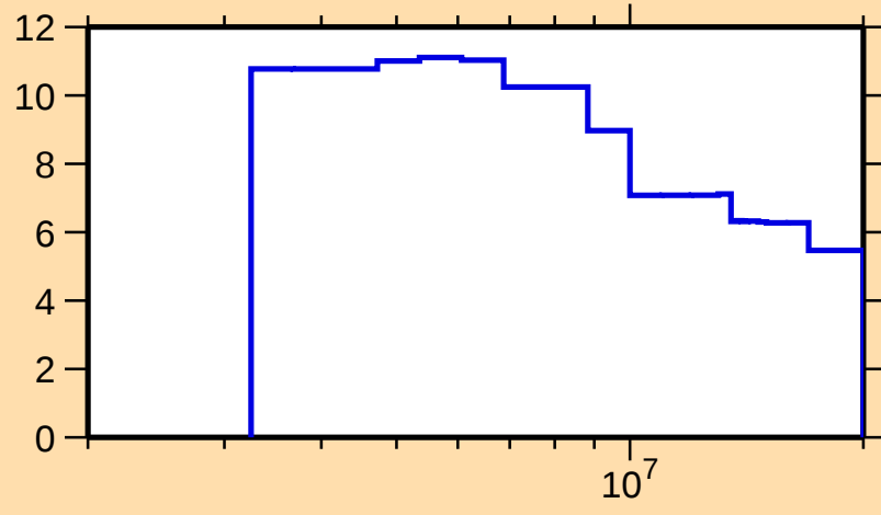
\Delta\sigma/\sigma vs. E for ^{34}\text{Si}(n,\text{tot.})
