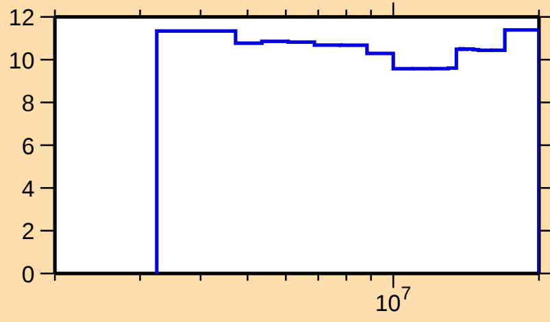
\Delta\sigma/\sigma vs. E for ^{34}\text{Si}(\text{n,nonel.})
