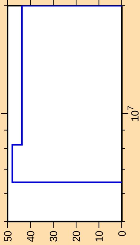
\Delta\sigma/\sigma vs. E for ^{34}\text{Si}(\text{n},\text{ncont.})
