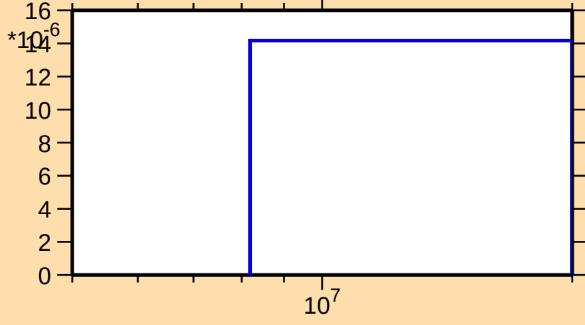
\sigma vs. E for ^{34}\text{Si}(n,\alpha)
