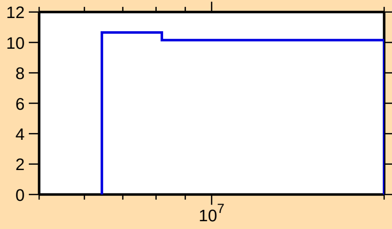
\Delta\sigma/\sigma vs. E for ^{34}\text{Si}(\text{n},\text{nonel.})
