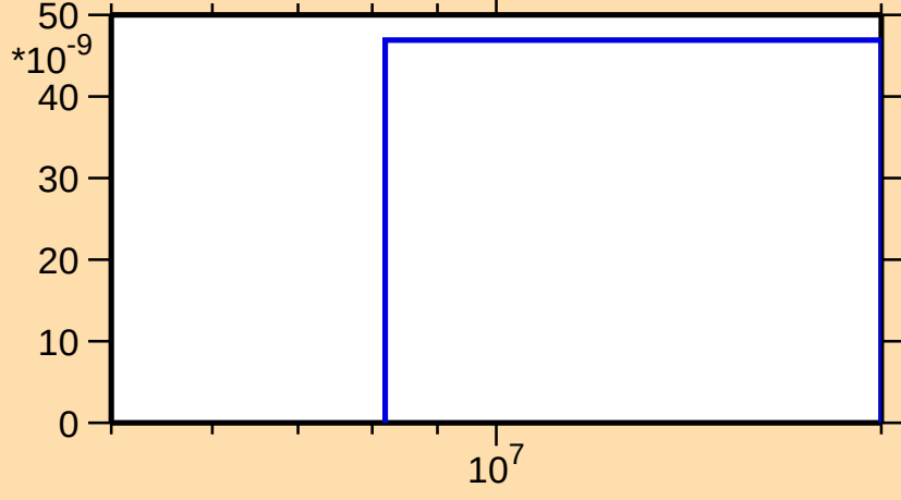
\sigma vs. E for ^{34}\text{Si}(n,d)
