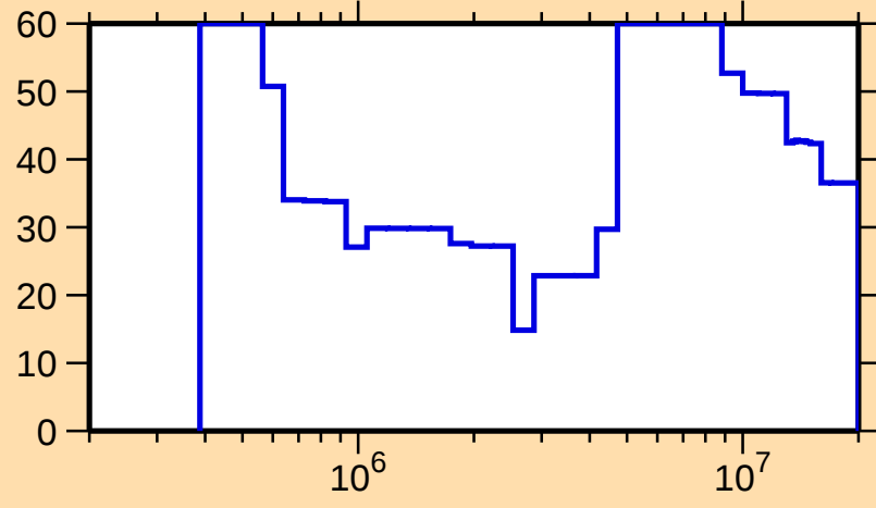
\Delta\sigma/\sigma vs. E for ^{132}\text{Sm}(n,\text{el.})
