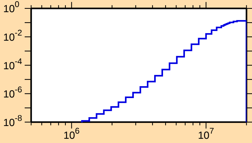
\sigma vs. E for ^{132}\text{Sm}(n,p\alpha)
