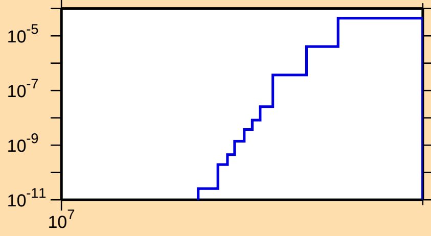
\sigma vs. E for ^{132}\text{Sm}(n,\text{pt})
