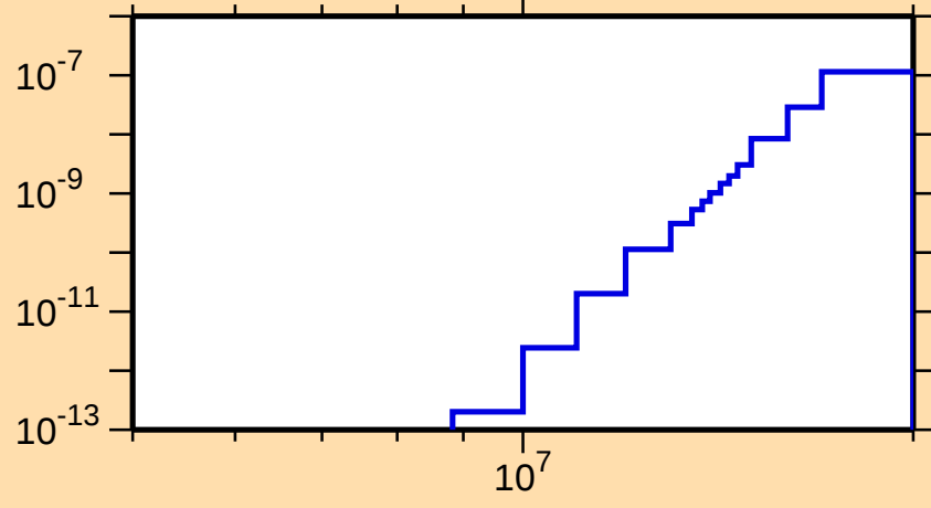
\sigma vs. E for ^{132}\text{Sm}(\text{mt117})
