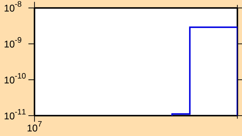
\sigma vs. E for ^{132}\text{Sm}(n,\text{nd})
