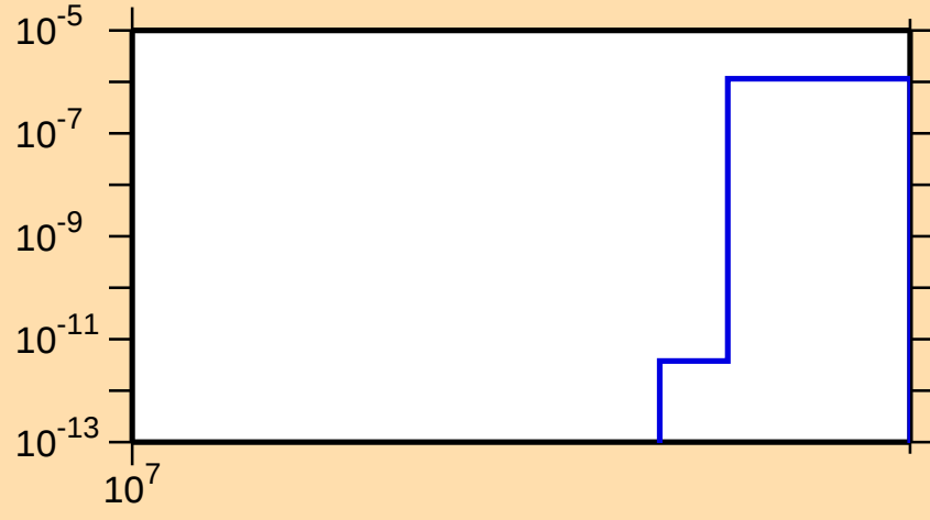
\sigma vs. E for ^{132}\text{Sm}(n,2np)
