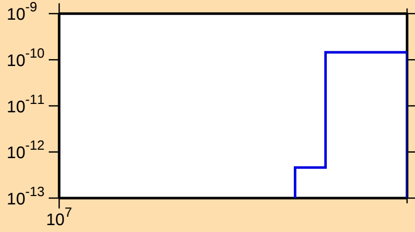
\sigma vs. E for ^{132}\text{Sm}(n,2n\alpha)
