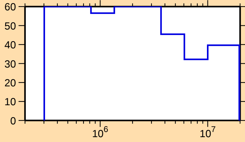
\Delta\sigma/\sigma vs. E for ^{132}\text{Sm}(n,\text{inel.})
