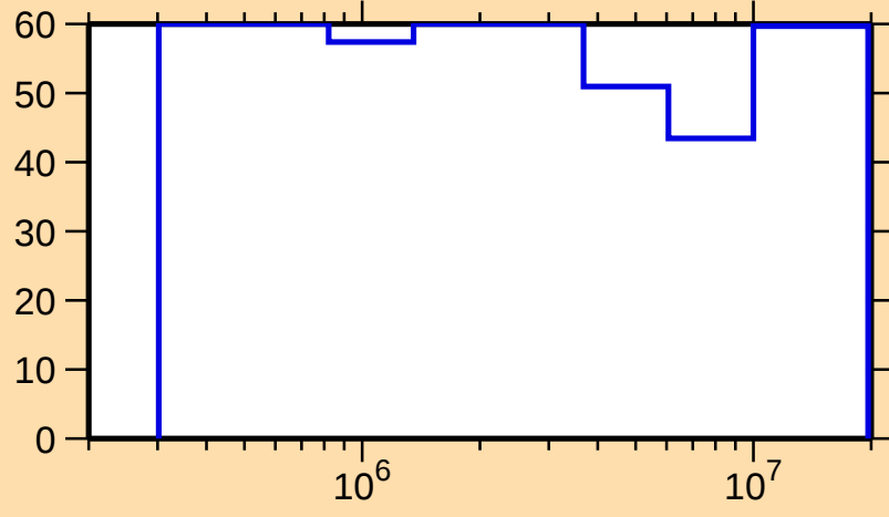
\Delta\sigma/\sigma vs. E for ^{132}\text{Sm}(n,n_1)
