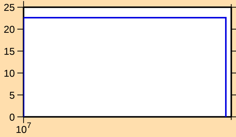
\Delta\sigma/\sigma vs. E for ^{132}\text{Sm}(n,\text{nonel.})
