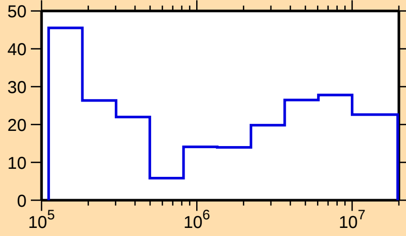
\Delta\sigma/\sigma vs. E for ^{132}\text{Sm}(n,\text{nonel.})
