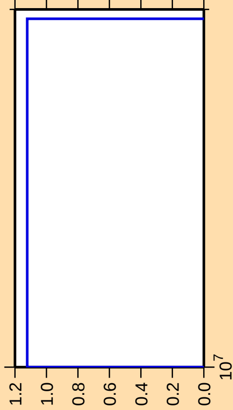
\Delta\sigma/\sigma vs. E for ^{132}\text{Sm}(n,2n\alpha)
