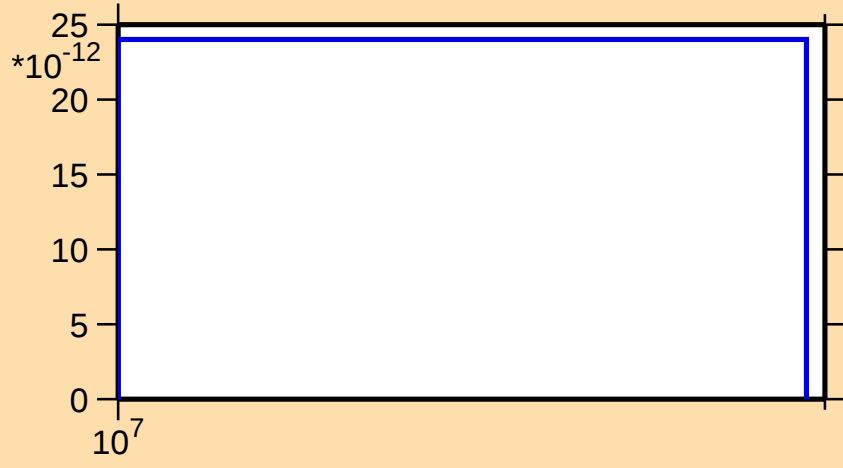
\sigma vs. E for ^{132}\text{Sm}(n,\text{nd})
