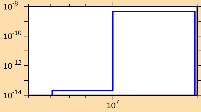
\sigma vs. E for ^{132}\text{Sm}(\text{mt117})
