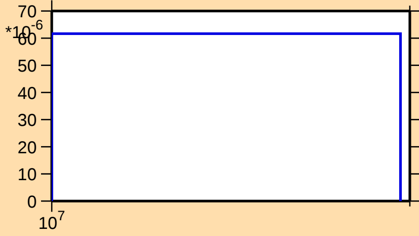
\sigma vs. E for ^{132}\text{Sm}(n,2n)
