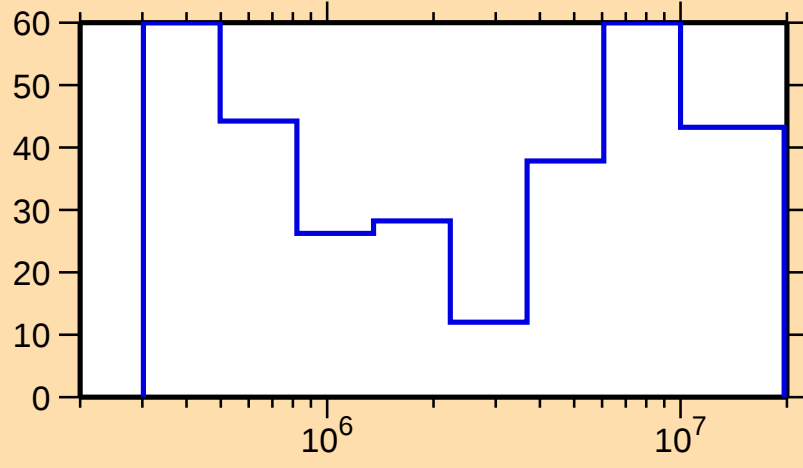
\Delta\sigma/\sigma vs. E for ^{132}\text{Sm}(n,\text{el.})
