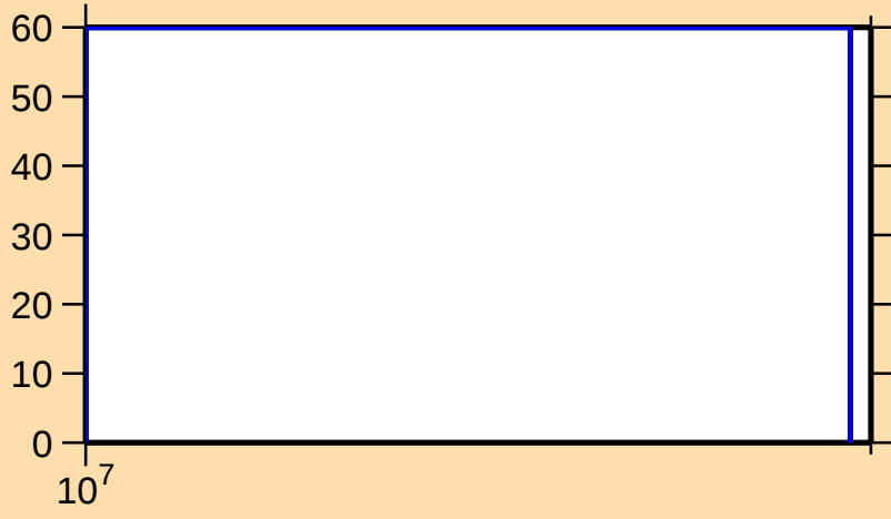
\Delta\sigma/\sigma vs. E for ^{132}\text{Sm}(n,2n)
