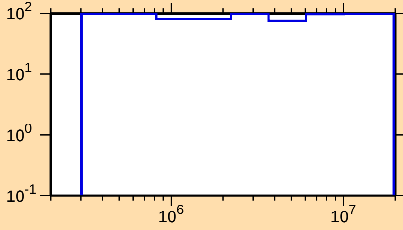
\Delta\sigma/\sigma vs. E for ^{132}\text{Sm}(n,n\text{cont.})
