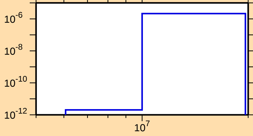
\sigma vs. E for ^{132}\text{Sm}(\text{mt } 45)
