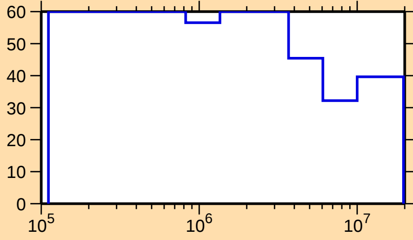
\Delta\sigma/\sigma vs. E for ^{132}\text{Sm}(n,\text{inel.})
