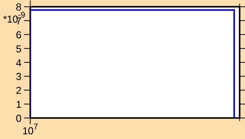
\sigma vs. E for ^{132}\text{Sm}(n,2np)
