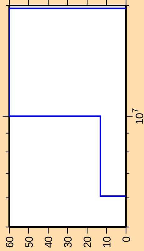
\Delta\sigma/\sigma vs. E for ^{132}\text{Sm}(\text{mt } 45)
