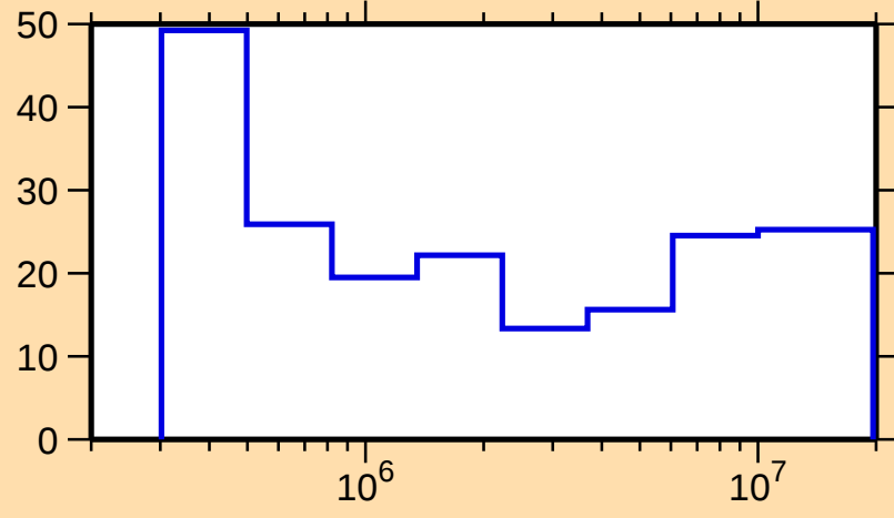
\Delta\sigma/\sigma vs. E for ^{132}\text{Sm}(n,\text{tot.})
