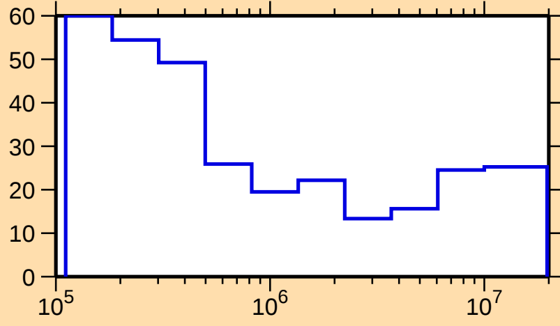
\Delta\sigma/\sigma vs. E for ^{132}\text{Sm}(n,\text{tot.})
