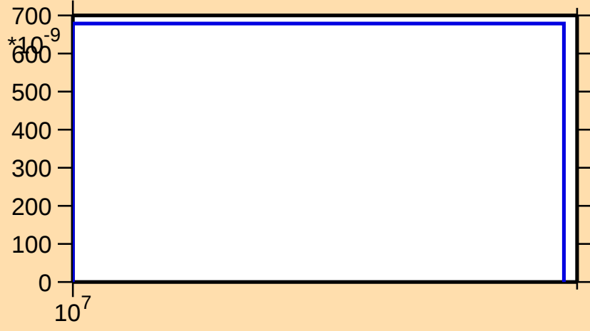
\sigma vs. E for ^{132}\text{Sm}(n,\text{pt})
