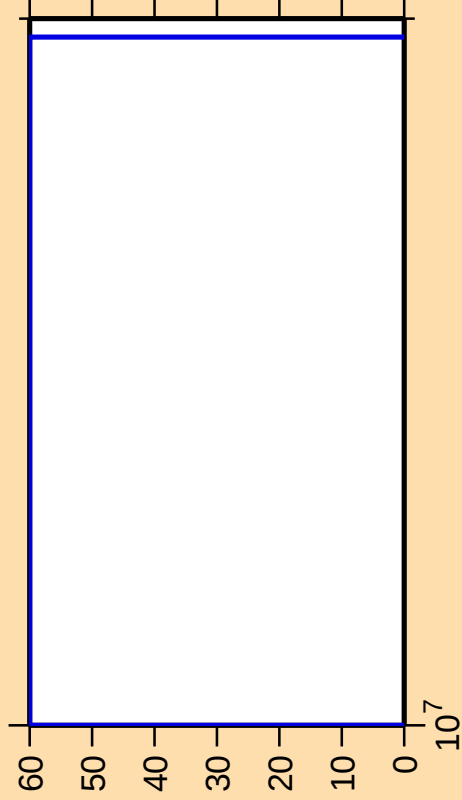
\Delta\sigma/\sigma vs. E for ^{132}\text{Sm}(n,2np)
