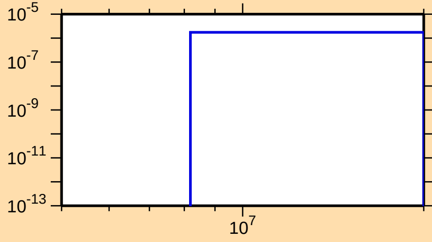
\sigma vs. E for ^{132}\text{Sm}(\text{mt } 45)
