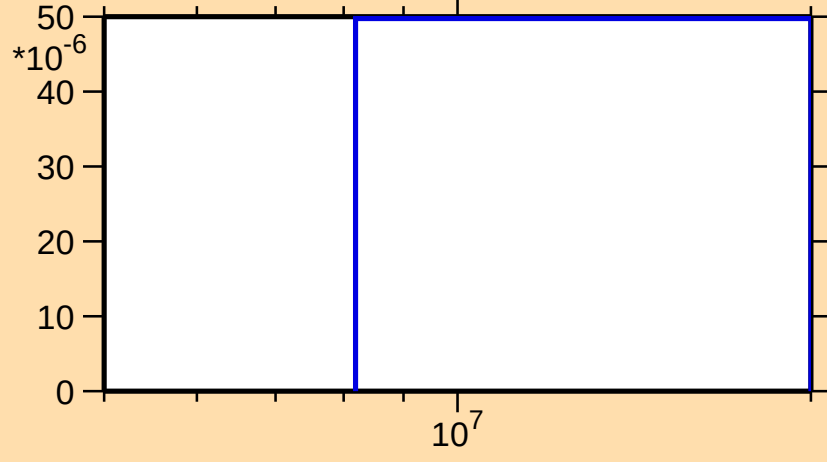
\sigma vs. E for ^{132}\text{Sm}(n,2n)
