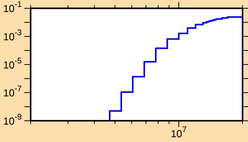
\sigma vs. E for ^{135}\text{Sm}(n,d)
