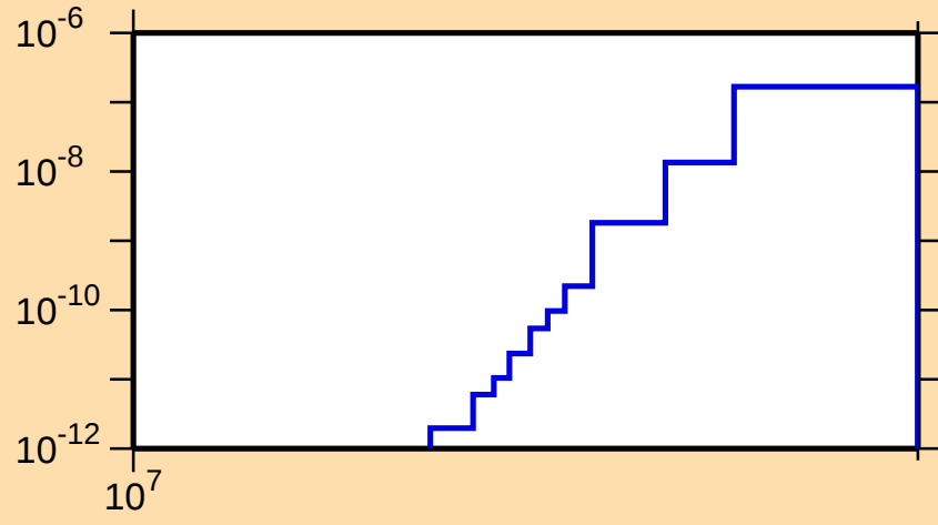
\sigma vs. E for ^{135}\text{Sm}(\text{mt } 34)
