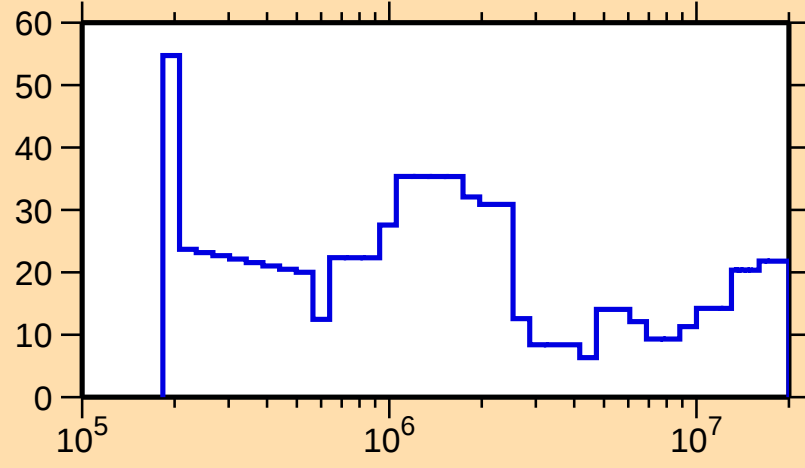
\Delta\sigma/\sigma vs. E for ^{135}\text{Sm}(n,\text{tot.})
