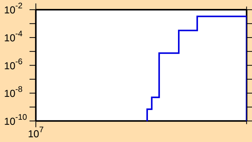
\sigma vs. E for ^{135}\text{Sm}(n,2np)
