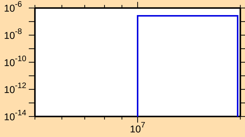
\sigma vs. E for ^{135}\text{Sm}(n,2n\alpha)
