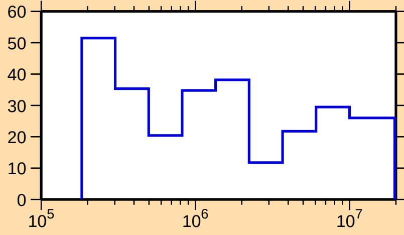
\Delta\sigma/\sigma vs. E for ^{135}\text{Sm}(n,\text{el.})
