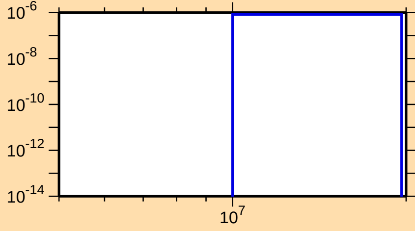
\sigma vs. E for ^{135}\text{Sm}(\text{mt } 45)
