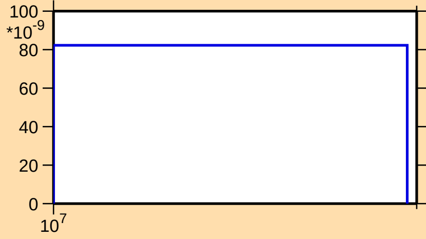
\sigma vs. E for ^{135}\text{Sm}(n,\text{nd})
