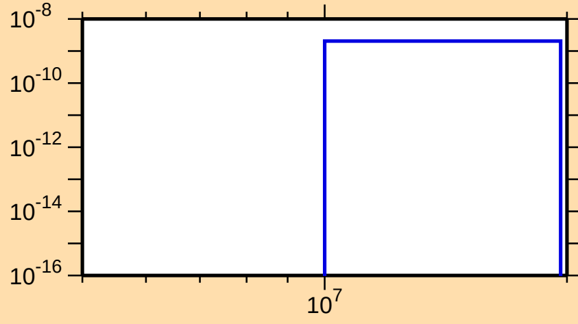
\sigma vs. E for ^{135}\text{Sm}(\text{mt117})
