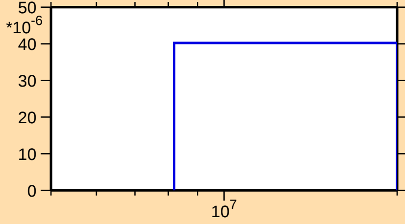
\sigma vs. E for ^{135}\text{Sm}(n,2np)
