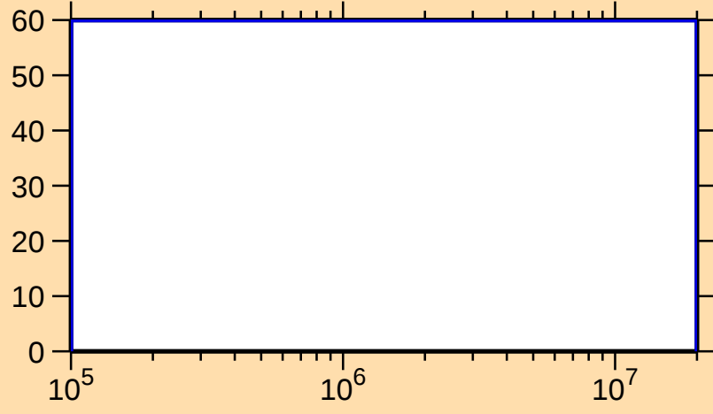
\Delta\sigma/\sigma vs. E for ^{135}\text{Sm}(n,n\text{cont.})
