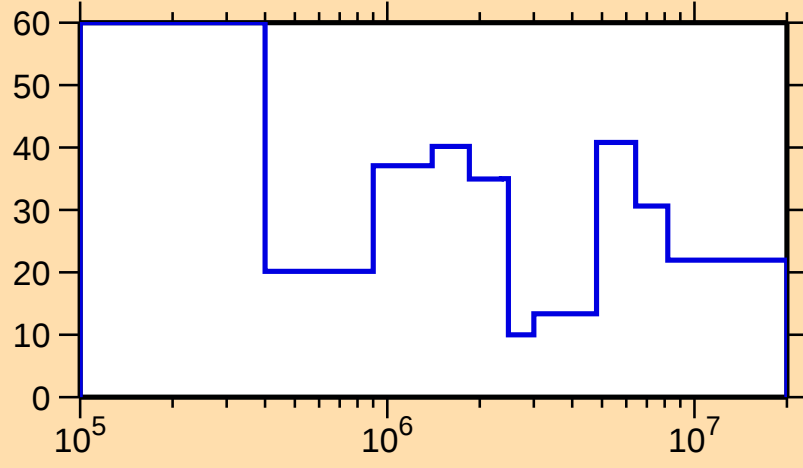
\Delta\sigma/\sigma vs. E for ^{135}\text{Sm}(n,\text{el.})
