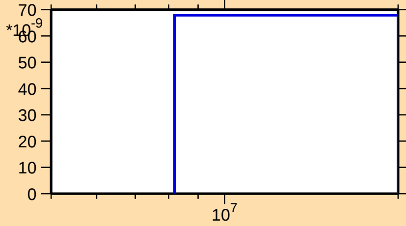
\sigma vs. E for ^{135}\text{Sm}(n,\text{nd})
