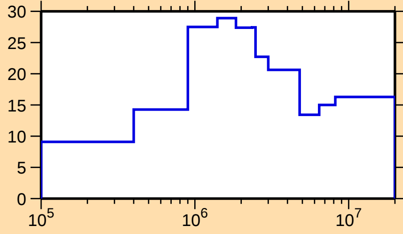
\Delta\sigma/\sigma vs. E for ^{135}\text{Sm}(n,n\text{onel.})
