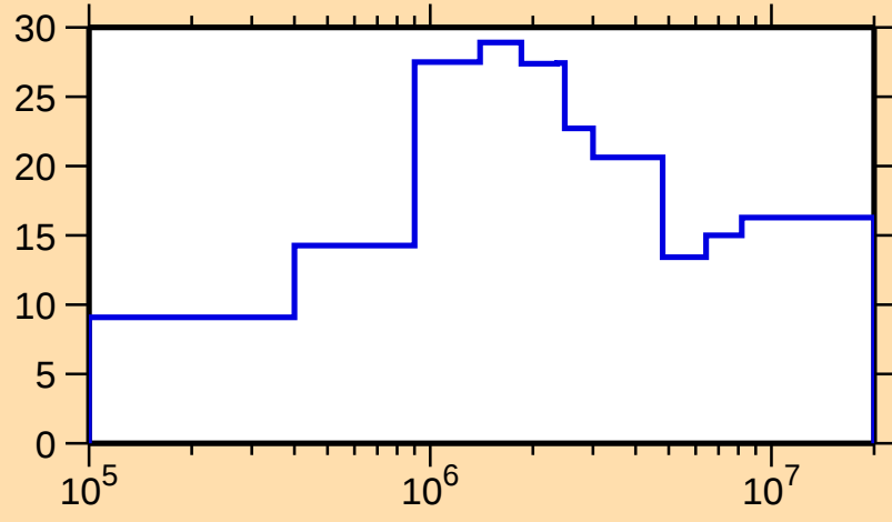
\Delta\sigma/\sigma vs. E for ^{135}\text{Sm}(n,\text{nonel.})
