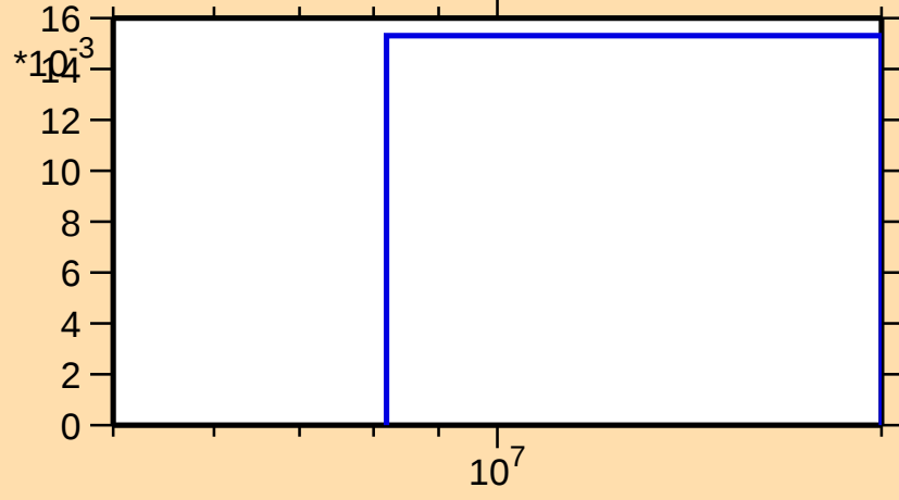
\sigma vs. E for ^{135}\text{Sm}(n,2n)
