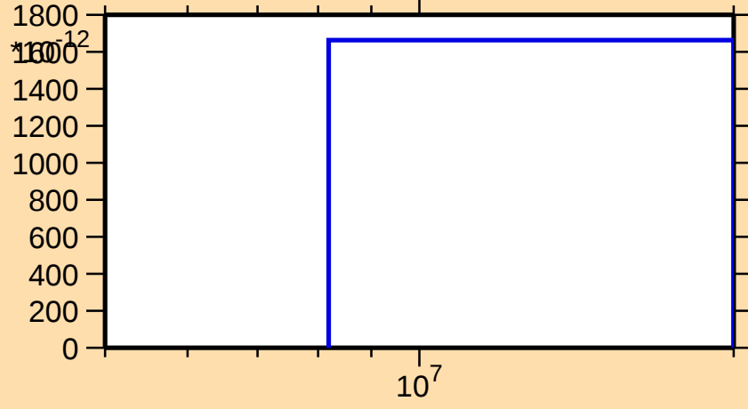
\sigma vs. E for ^{135}\text{Sm}(\text{mt117})
