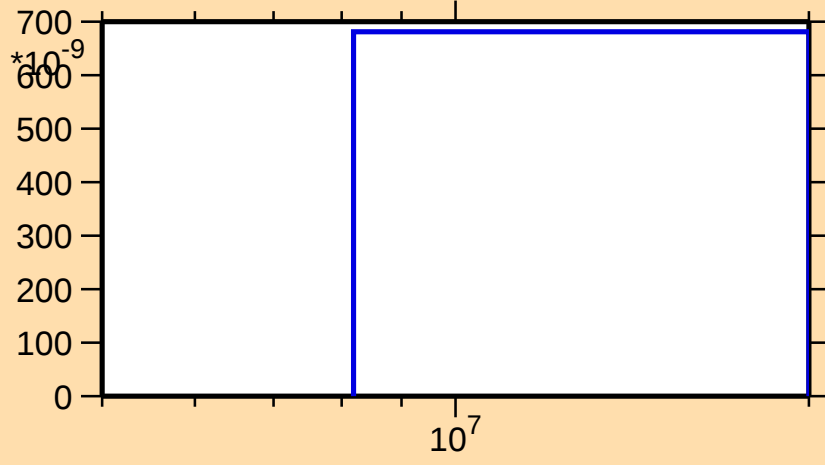
\sigma vs. E for ^{135}\text{Sm}(\text{mt } 45)
