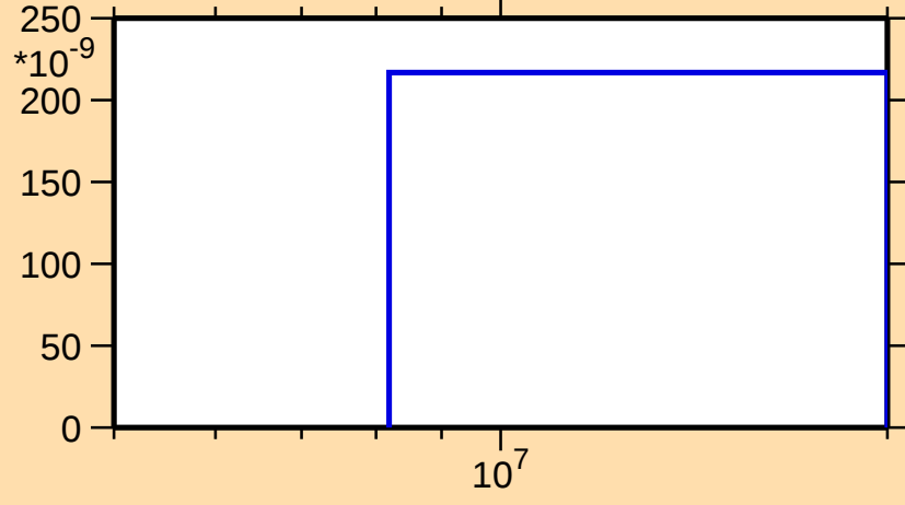
\sigma vs. E for ^{135}\text{Sm}(n,2n\alpha)
