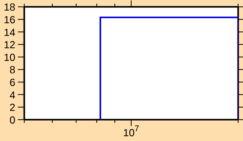
\Delta\sigma/\sigma vs. E for ^{135}\text{Sm}(n,\text{tot.})
