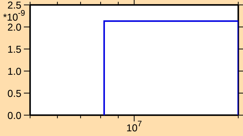
\sigma vs. E for ^{135}\text{Sm}(\text{mt } 34)
