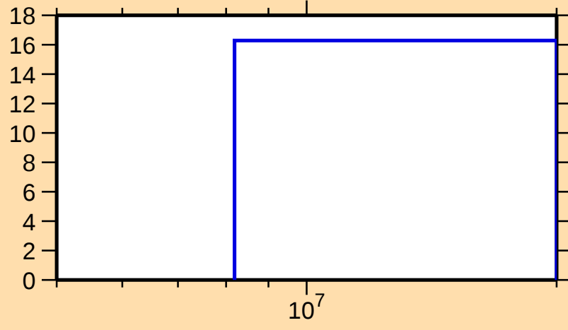
\Delta\sigma/\sigma vs. E for ^{135}\text{Sm}(n,\text{nonel.})
