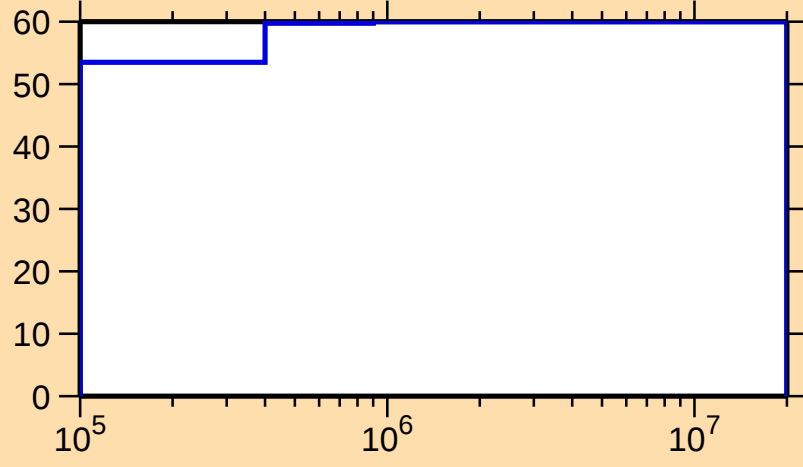
\Delta\sigma/\sigma vs. E for ^{135}\text{Sm}(n,n_1)
