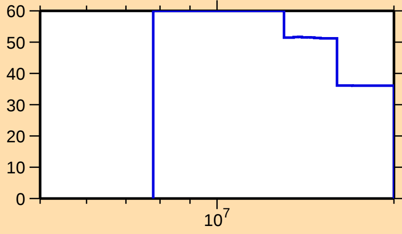
\Delta\sigma/\sigma vs. E for ^{141}\text{Sm}(n,2n)
