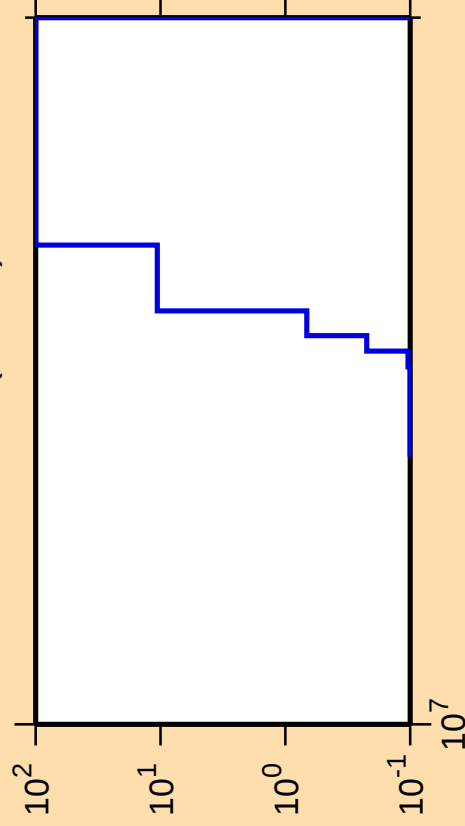
\Delta\sigma/\sigma vs. E for ^{141}\text{Sm}(\text{mt } 45)
