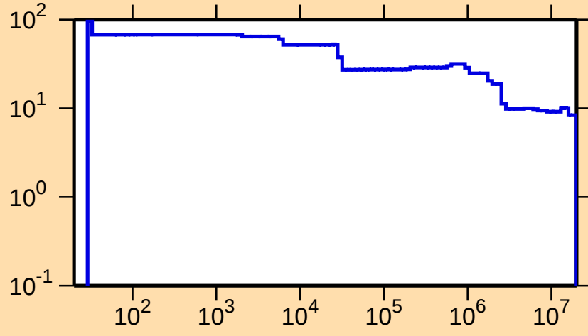
\Delta\sigma/\sigma vs. E for ^{141}\text{Sm}(n,\text{nonel.})
