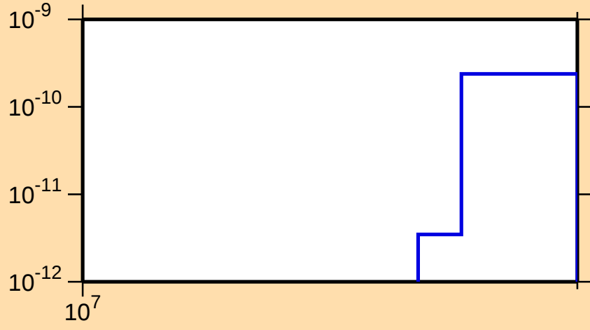
\sigma vs. E for ^{141}\text{Sm}(\text{mt } 34)
