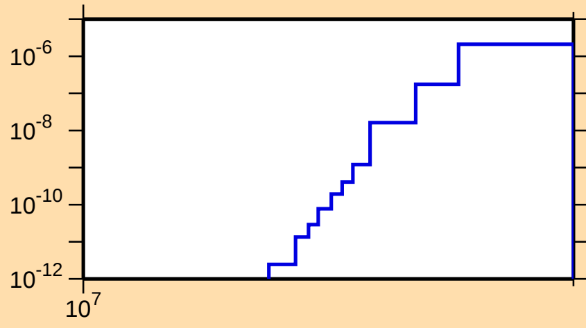
\sigma vs. E for ^{141}\text{Sm}(n,2n\alpha)
