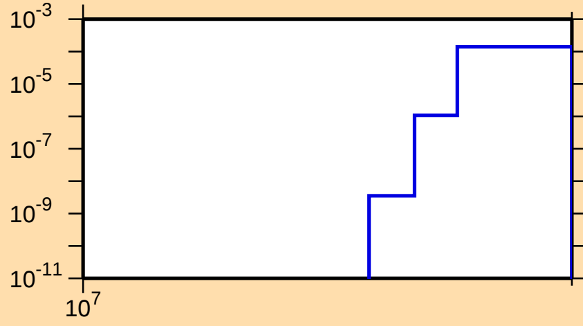
\sigma vs. E for ^{141}\text{Sm}(n,2np)
