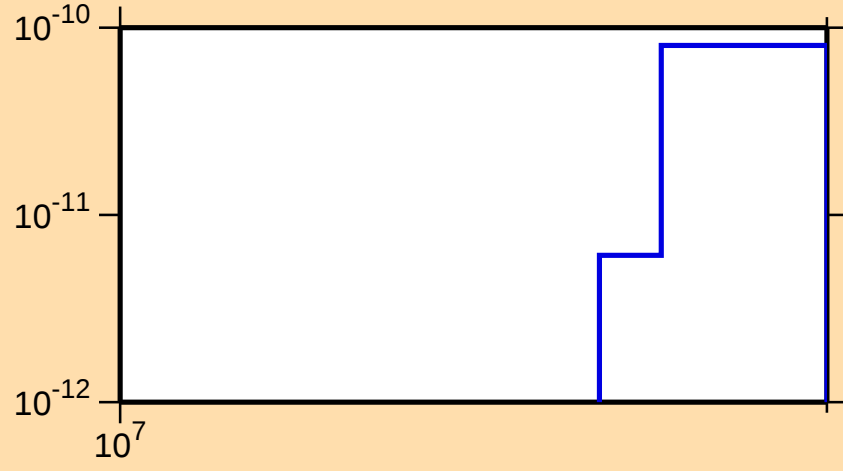
\sigma vs. E for ^{141}\text{Sm}(\text{mt117})
