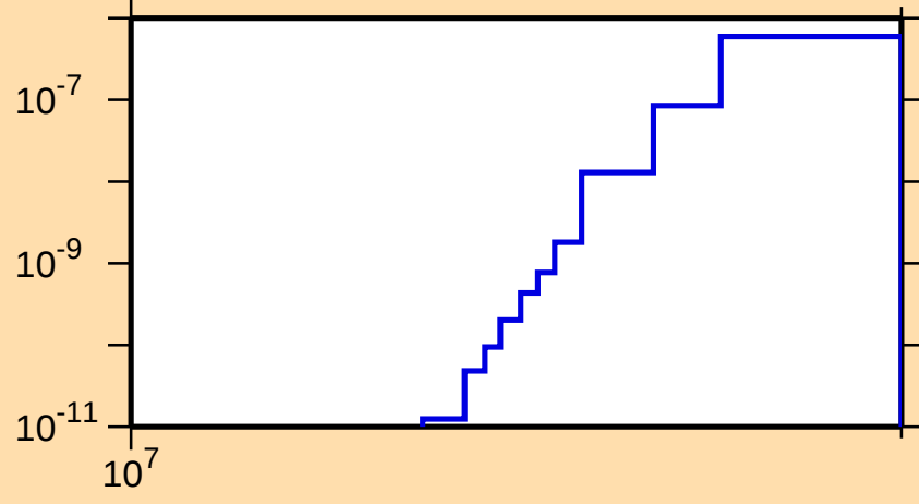
\sigma vs. E for ^{141}\text{Sm}(n,\text{pd})
