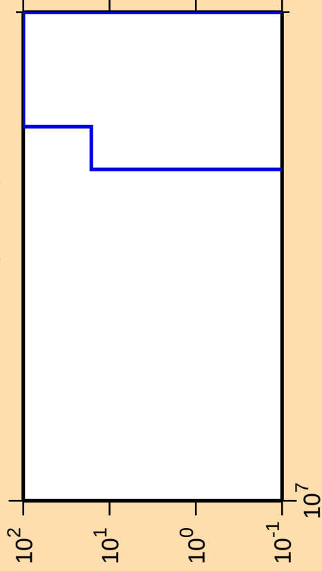
\Delta\sigma/\sigma vs. E for ^{141}\text{Sm}(\text{mt } 34)
