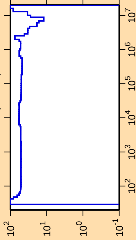
\Delta\sigma/\sigma vs. E for ^{141}\text{Sm}(n,\text{inel.})
