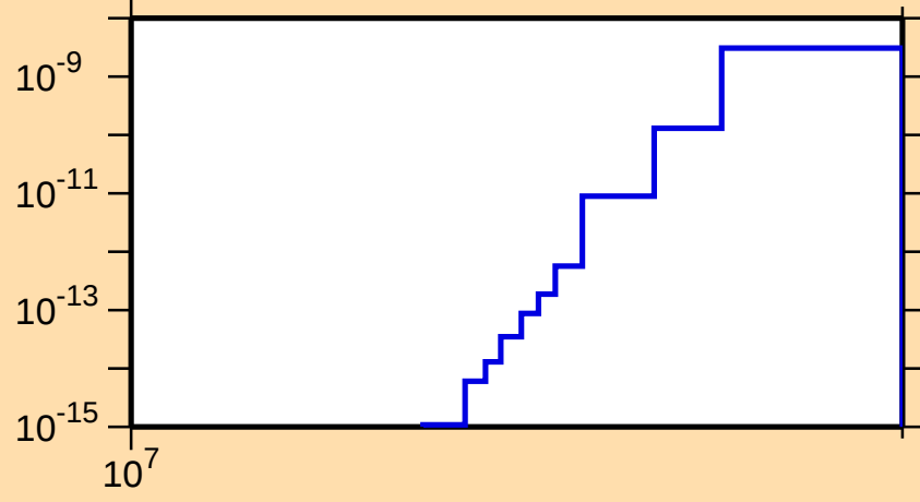
\sigma vs. E for ^{141}\text{Sm}(\text{mt } 45)
