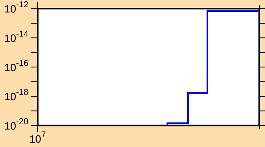
\sigma vs. E for ^{141}\text{Sm}(n,nt)
