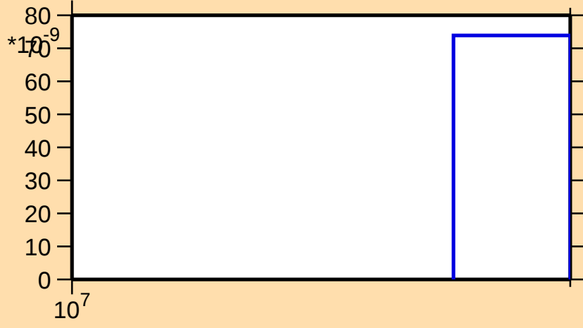
\sigma vs. E for ^{141}\text{Sm}(n,3n)
