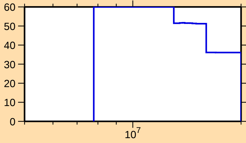
\Delta\sigma/\sigma vs. E for ^{141}\text{Sm}(n,2n)
