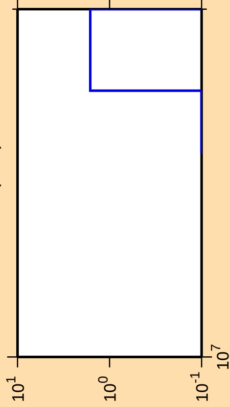
\Delta\sigma/\sigma vs. E for ^{141}\text{Sm}(n,nt)
