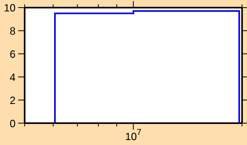
\Delta\sigma/\sigma vs. E for ^{141}\text{Sm}(n,\text{nonel.})
