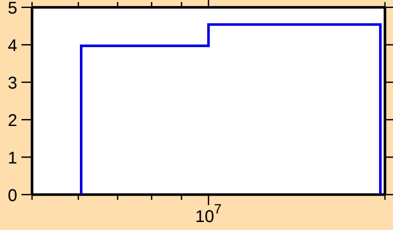
\Delta\sigma/\sigma vs. E for ^{141}\text{Sm}(n,\text{tot.})
