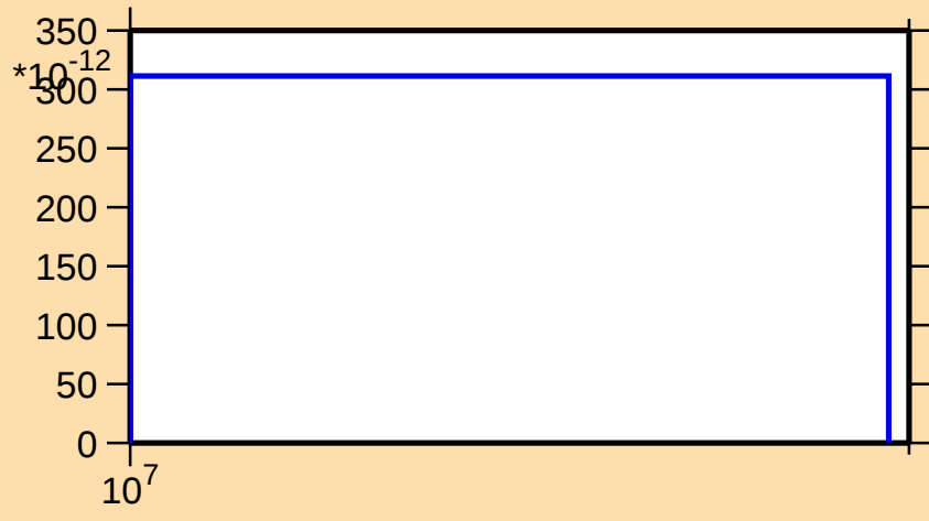
\sigma vs. E for ^{141}\text{Sm}(n,\text{pt})
