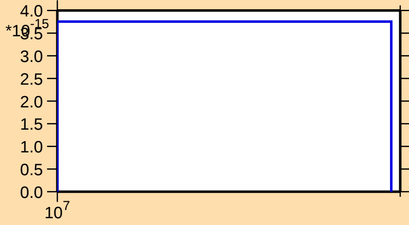
\sigma vs. E for ^{141}\text{Sm}(n,\text{nt})
