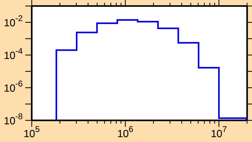
\sigma vs. E for ^{141}\text{Sm}(n,n_4)
