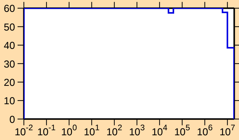
\Delta\sigma/\sigma vs. E for ^{141}\text{Sm}(n,p)
