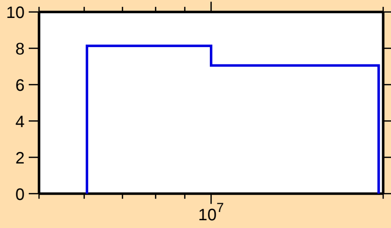
\Delta\sigma/\sigma vs. E for ^{141}\text{Sm}(n,\text{el.})
