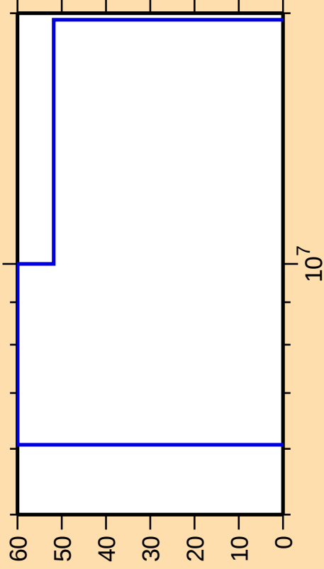
\Delta\sigma/\sigma vs. E for ^{141}\text{Sm}(n,2n)
