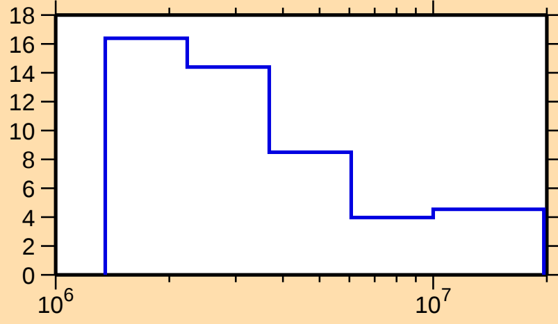
\Delta\sigma/\sigma vs. E for ^{141}\text{Sm}(n,\text{tot.})
