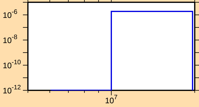
\sigma vs. E for ^{141}\text{Sm}(n,\text{He}3)
