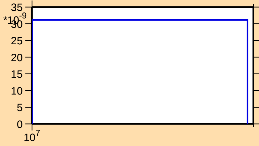
\sigma vs. E for ^{141}\text{Sm}(n,2n\alpha)
