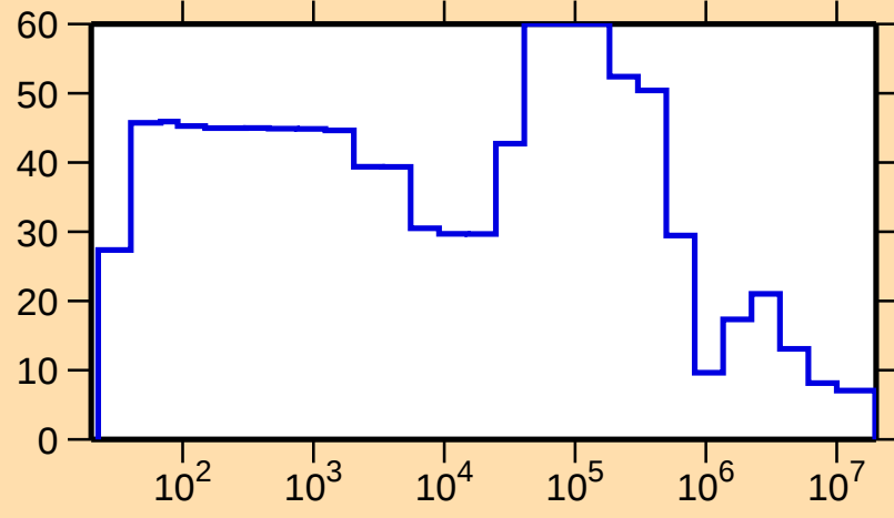
\Delta\sigma/\sigma vs. E for ^{141}\text{Sm}(n,\text{el.})
