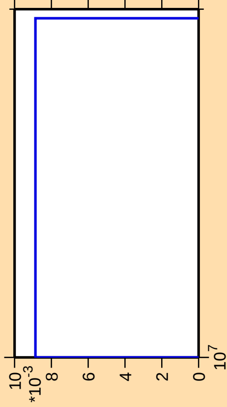
\Delta\sigma/\sigma vs. E for ^{141}\text{Sm}(n,\text{nt})
