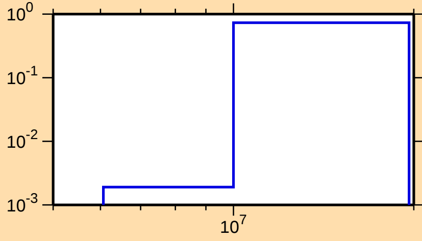
\sigma vs. E for ^{141}\text{Sm}(n,2n)
