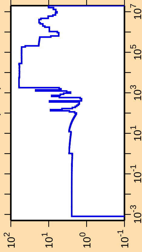
\Delta\sigma/\sigma vs. E for ^{146}\text{Sm}(n,\text{el.})
