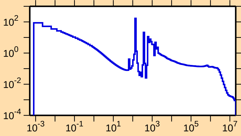
\sigma vs. E for ^{146}\text{Sm}(n,\gamma)
