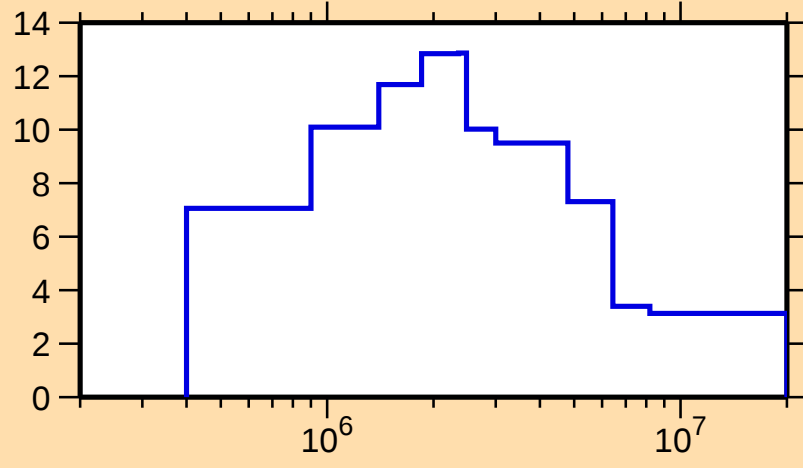
\Delta\sigma/\sigma vs. E for ^{146}\text{Sm}(n,\text{tot.})
