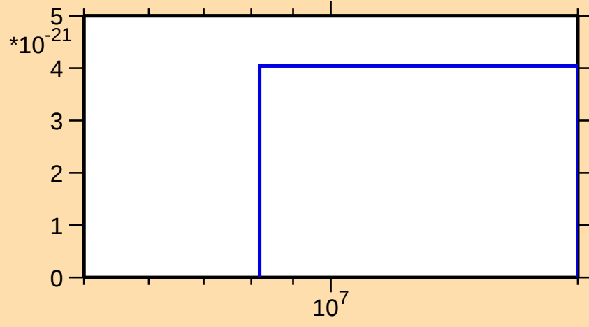
\sigma vs. E for ^{146}\text{Sm}(\text{mt } 11)
