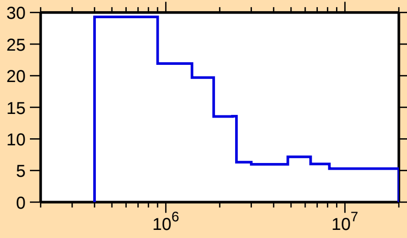
\Delta\sigma/\sigma vs. E for ^{146}\text{Sm}(n,\text{nonel.})
