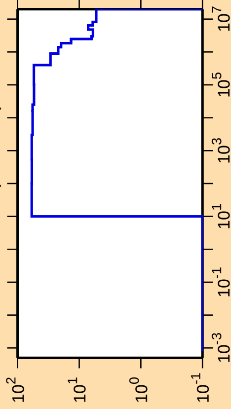
\Delta\sigma/\sigma vs. E for ^{146}\text{Sm}(n,\text{nonel.})
