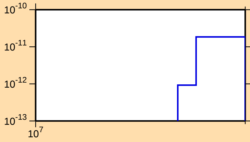
\sigma vs. E for ^{147}\text{Sm} (mt 45)
