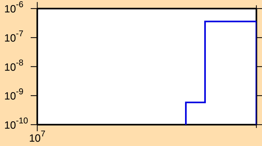
\sigma vs. E for ^{147}\text{Sm}(n,\text{nt})
