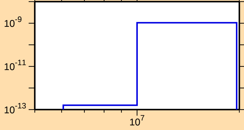
\sigma vs. E for ^{147}\text{Sm}(n,p\alpha)
