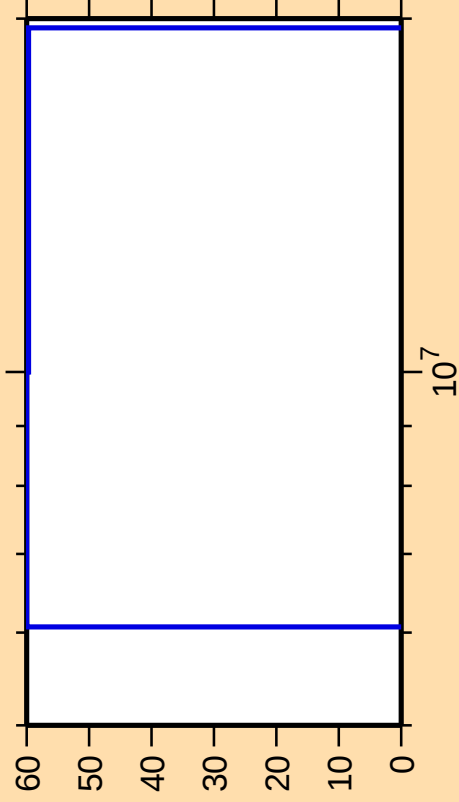
\Delta\sigma/\sigma vs. E for ^{147}\text{Sm}(n,\alpha)
