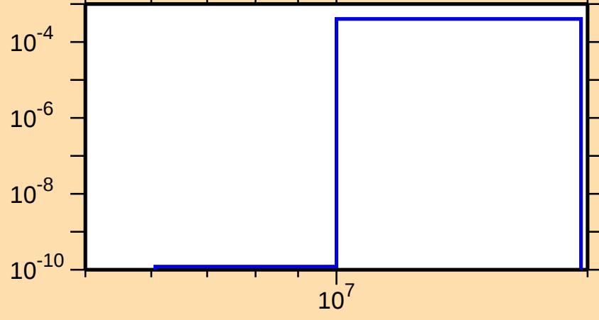
\sigma vs. E for ^{147}\text{Sm}(n,t)
