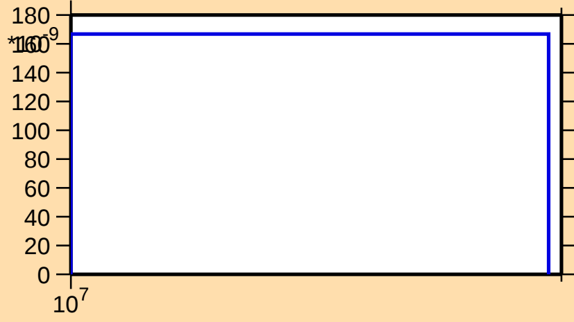
\sigma vs. E for ^{147}\text{Sm}(n,\text{nd})
