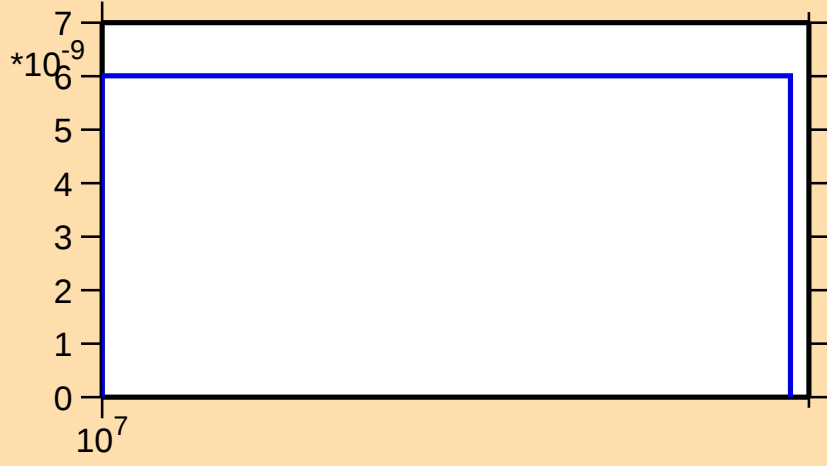
\sigma vs. E for ^{147}\text{Sm}(n,\text{He}3)
