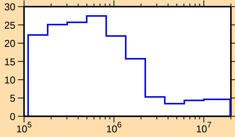
\Delta\sigma/\sigma vs. E for ^{147}\text{Sm}(n,\text{nonel.})
