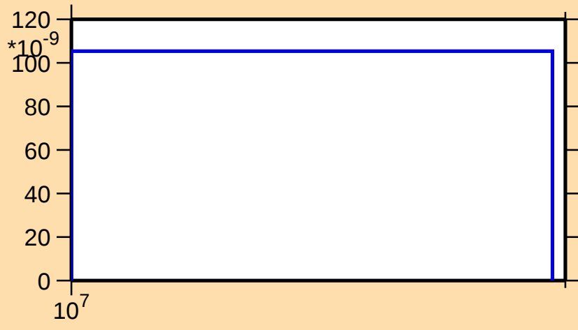
\sigma vs. E for ^{147}\text{Sm}(n,2np)
