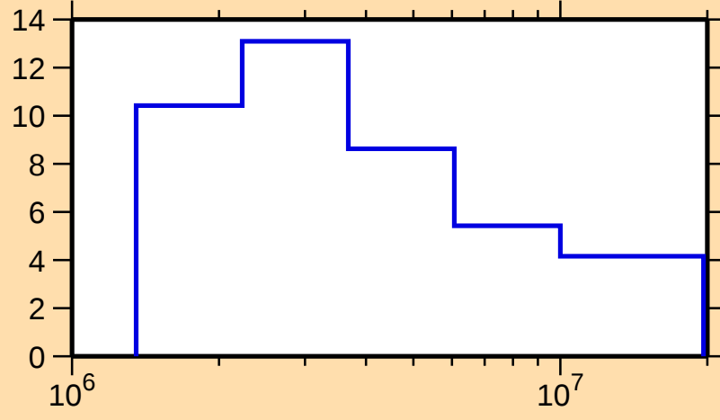
\Delta\sigma/\sigma vs. E for ^{147}\text{Sm}(n,\text{el.})
