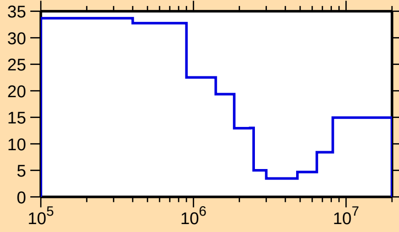
\Delta\sigma/\sigma vs. E for ^{147}\text{Sm}(n,\text{inel.})
