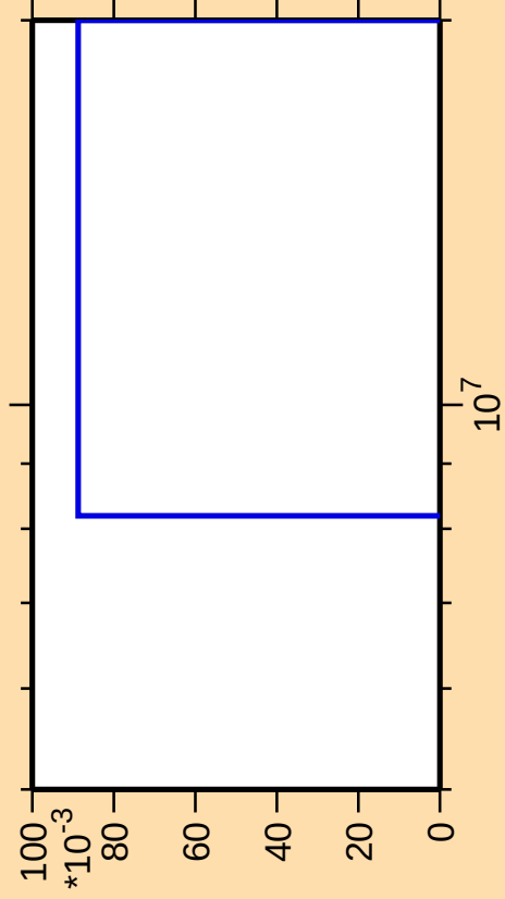
\Delta\sigma/\sigma vs. E for ^{147}\text{Sm}(\text{mt } 34)
