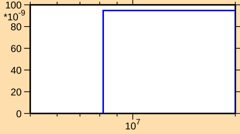
\sigma vs. E for ^{147}\text{Sm}(n,2np)
