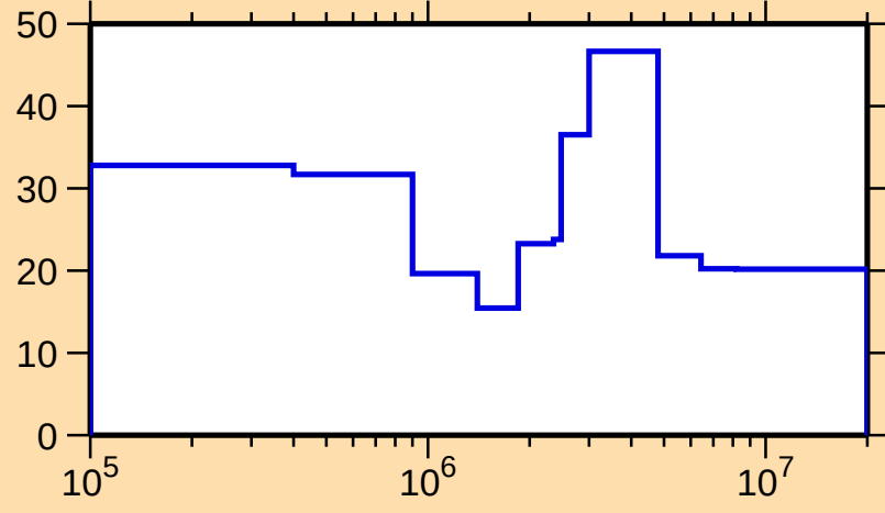
\Delta\sigma/\sigma vs. E for ^{147}\text{Sm}(n,n_1)
