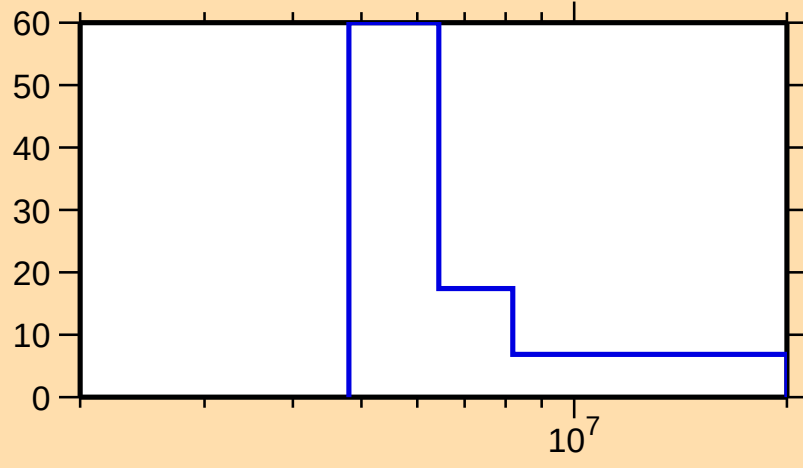
\Delta\sigma/\sigma vs. E for ^{147}\text{Sm}(n,2n)
