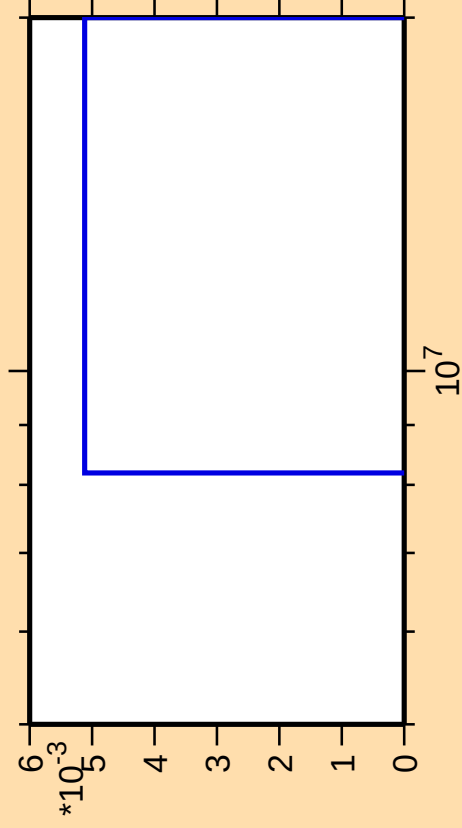
\Delta\sigma/\sigma vs. E for ^{147}\text{Sm}(n,\text{pd})
