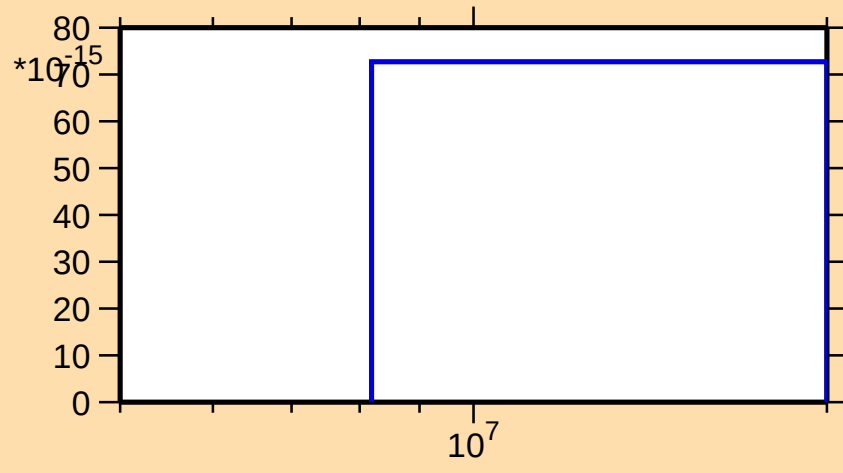
\sigma vs. E for ^{147}\text{Sm}(n,\text{pt})
