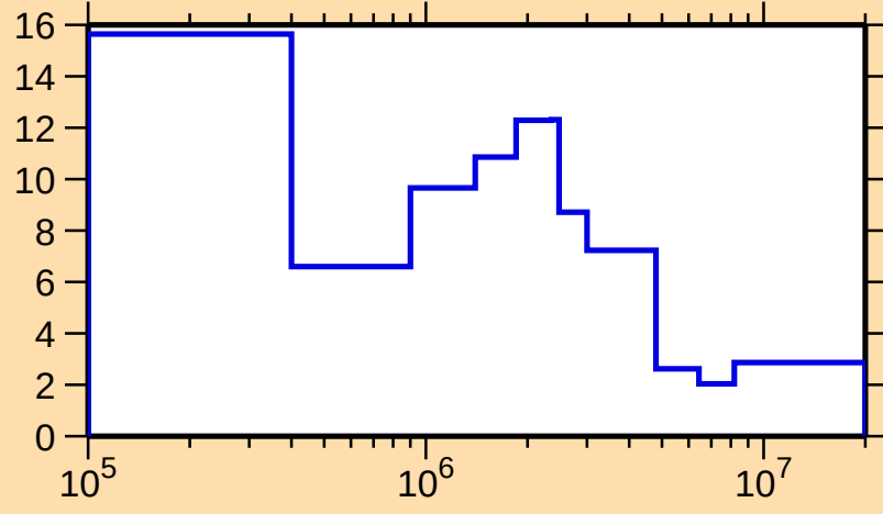
\Delta\sigma/\sigma vs. E for ^{147}\text{Sm}(n,\text{tot.})
