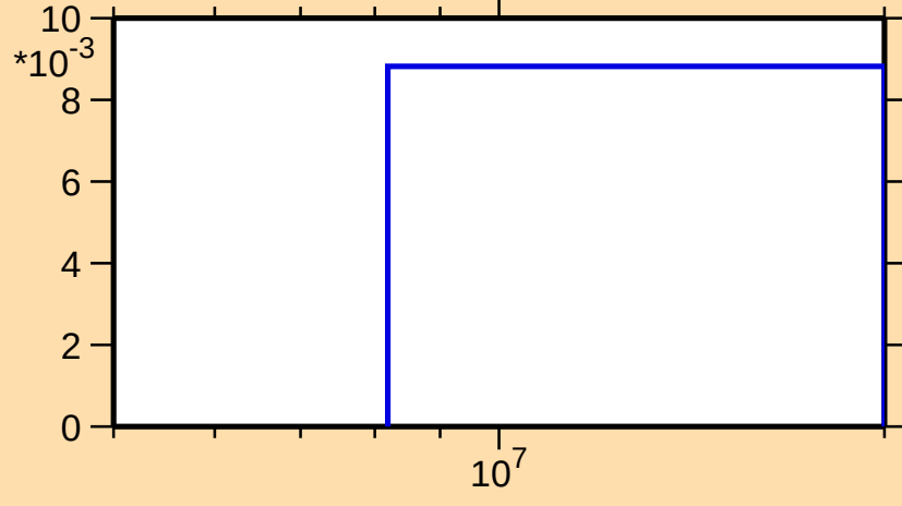
\sigma vs. E for ^{147}\text{Sm}(n,3n)
