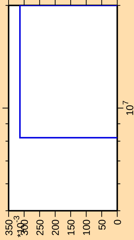
\Delta\sigma/\sigma vs. E for ^{147}\text{Sm}(\text{mt } 45)
