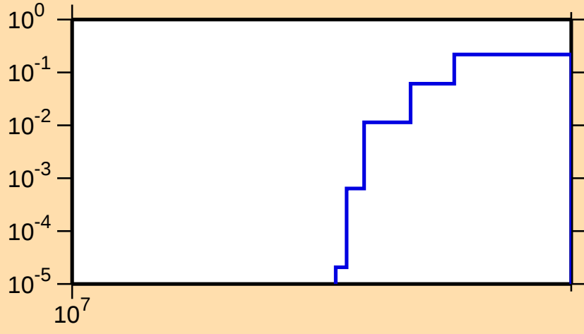
\sigma vs. E for ^{148}\text{Sm}(n,3n)
