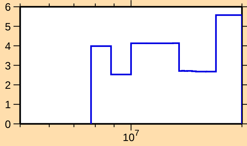
\Delta\sigma/\sigma vs. E for ^{148}\text{Sm}(n,\text{tot.})
