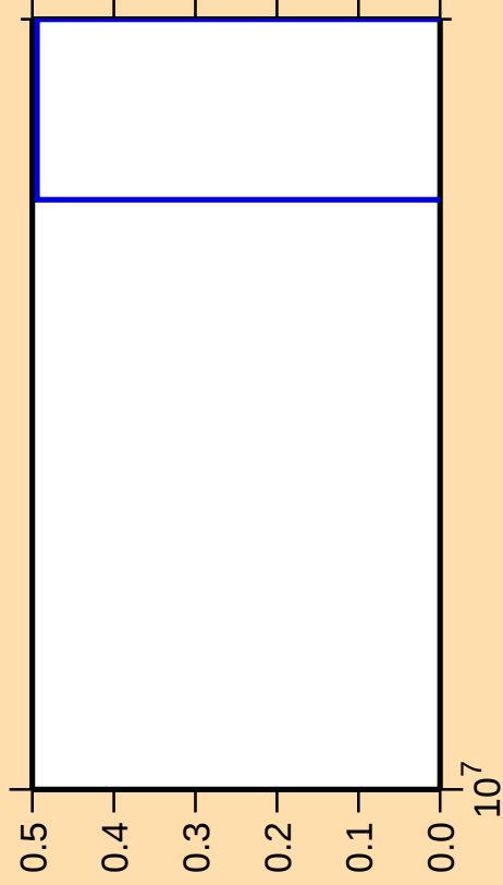
\Delta\sigma/\sigma vs. E for ^{148}\text{Sm}(n,\text{pd})
