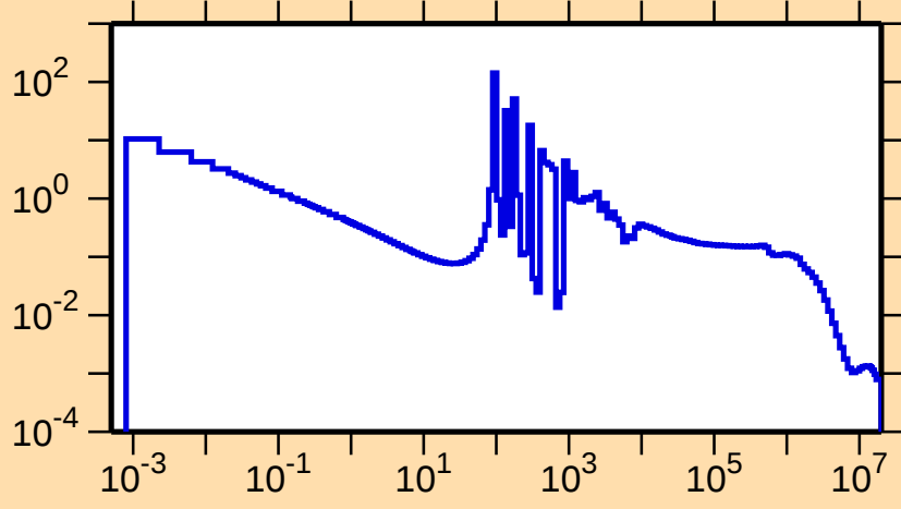
\sigma vs. E for ^{148}\text{Sm}(n,\gamma)
