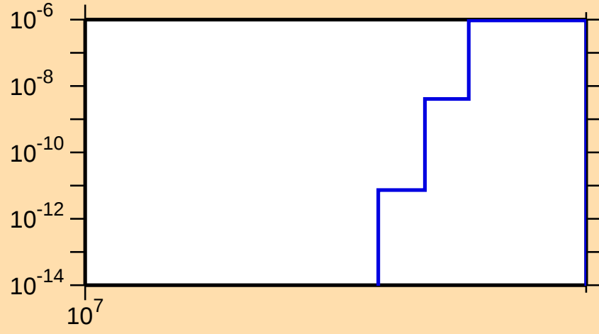
\sigma vs. E for ^{148}\text{Sm}(n,\text{nd})
