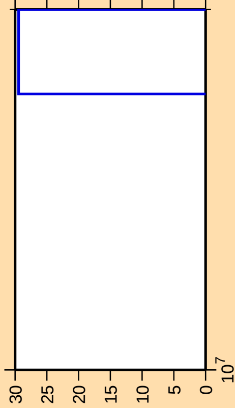
\Delta\sigma/\sigma vs. E for ^{148}\text{Sm}(\text{mt117})
