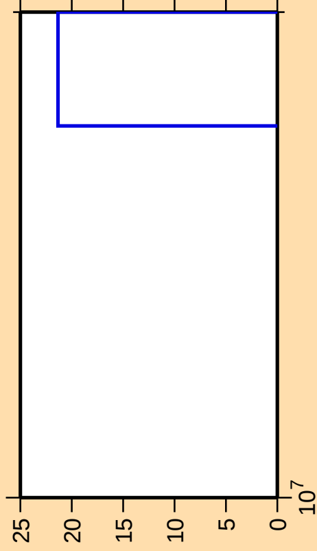
\Delta\sigma/\sigma vs. E for ^{148}\text{Sm}(\text{mt } 45)
