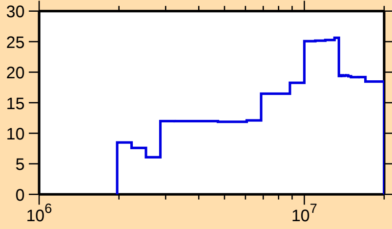
\Delta\sigma/\sigma vs. E for ^{148}\text{Sm}(n,\text{inel.})
