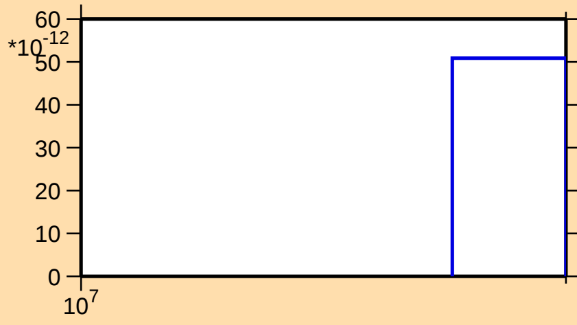
\sigma vs. E for ^{148}\text{Sm}(n,3n\alpha)
