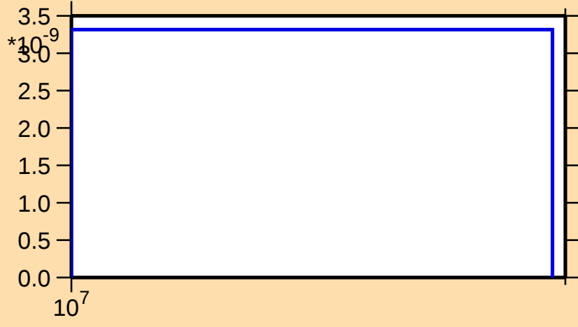
\sigma vs. E for ^{148}\text{Sm}(n,2np)
