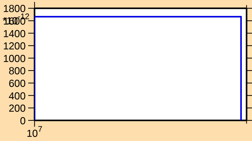
\sigma vs. E for ^{148}\text{Sm}(n,nt)
