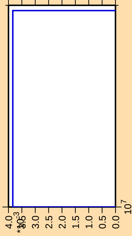
\Delta\sigma/\sigma vs. E for ^{148}\text{Sm}(n,\text{pd})
