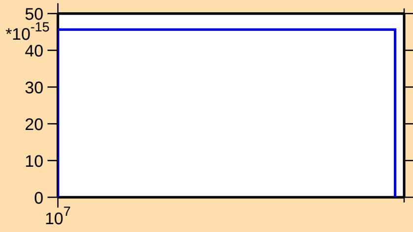
\sigma vs. E for ^{148}\text{Sm}(\text{mt } 45)
