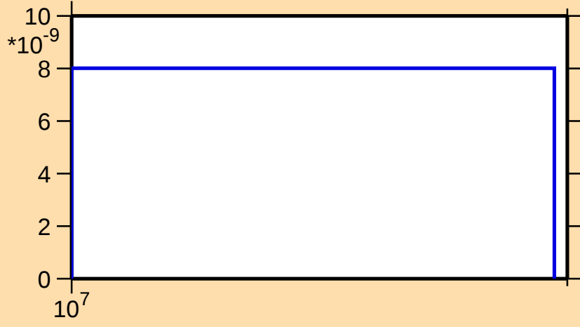
\sigma vs. E for ^{148}\text{Sm}(n,\text{nd})
