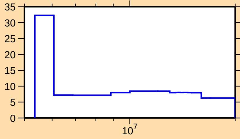
\Delta\sigma/\sigma vs. E for ^{149}\text{Sm}(n,2n)
