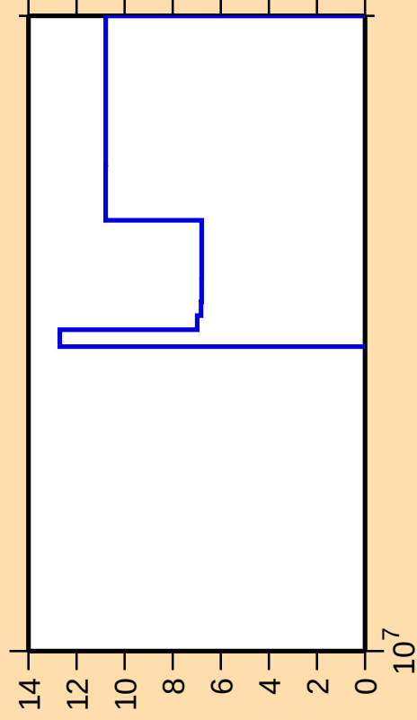
\Delta\sigma/\sigma vs. E for ^{149}\text{Sm}(n,3n)
