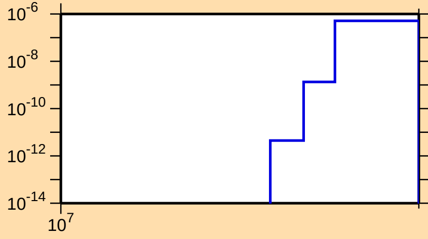
\sigma vs. E for ^{149}\text{Sm}(n,nt)
