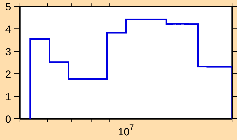
\Delta\sigma/\sigma vs. E for ^{149}\text{Sm}(n,\text{tot.})
