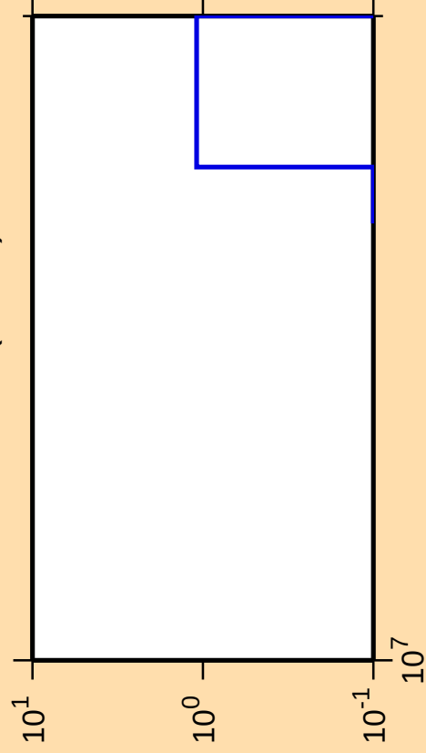
\Delta\sigma/\sigma vs. E for ^{149}\text{Sm}(\text{mt } 34)
