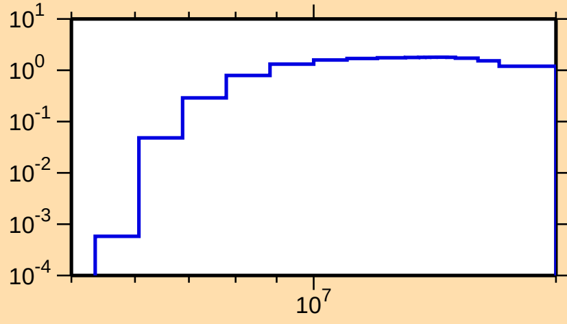
\sigma vs. E for ^{149}\text{Sm}(n,2n)
