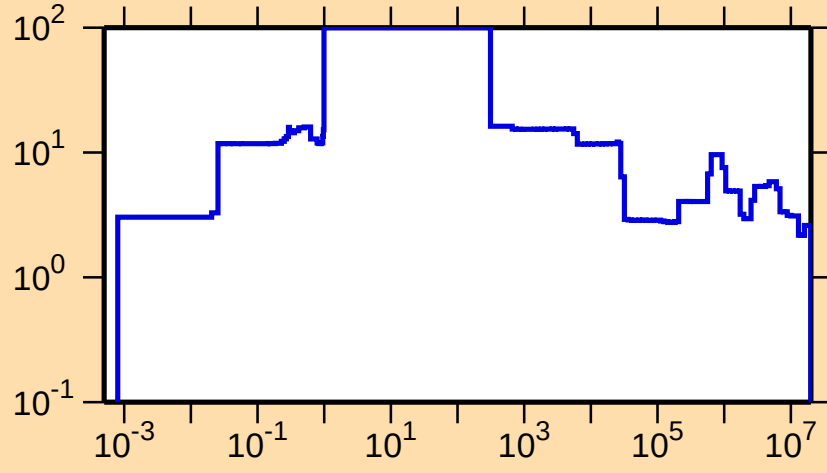
\Delta\sigma/\sigma vs. E for ^{149}\text{Sm}(n,\text{nonel.})
