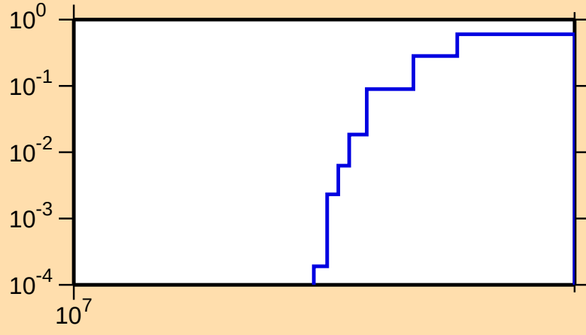
\sigma vs. E for ^{149}\text{Sm}(n,3n)
