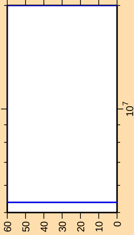
\Delta\sigma/\sigma vs. E for ^{149}\text{Sm}(n,\gamma)
