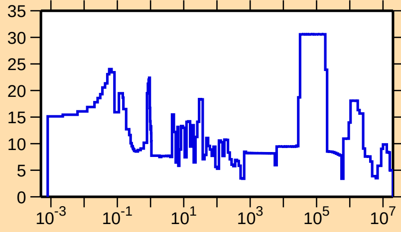
\Delta\sigma/\sigma vs. E for ^{149}\text{Sm}(n,\text{el.})
