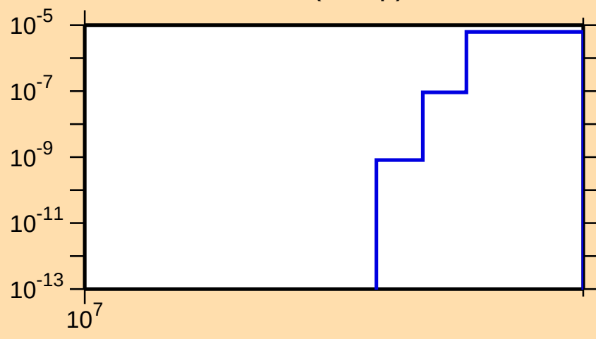
\sigma vs. E for ^{149}\text{Sm}(n,2np)
