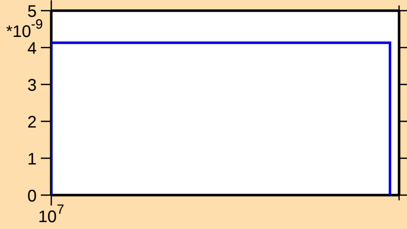
\sigma vs. E for ^{149}\text{Sm}(n,\text{nt})
