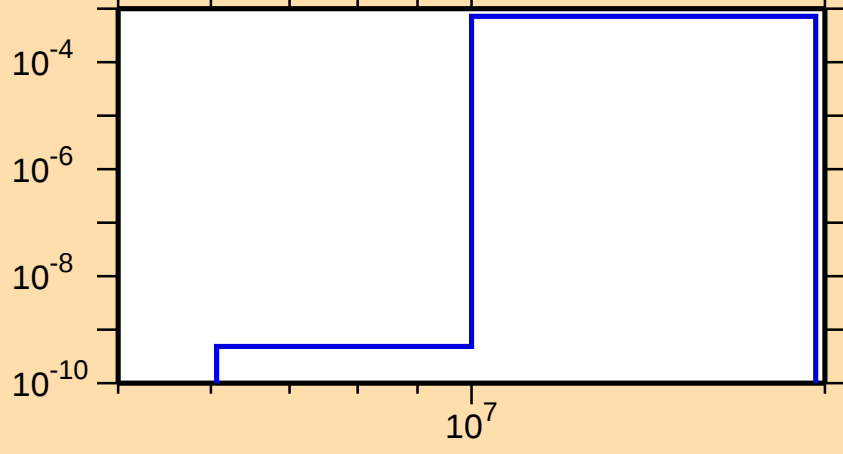
\sigma vs. E for ^{149}\text{Sm}(n,d)
