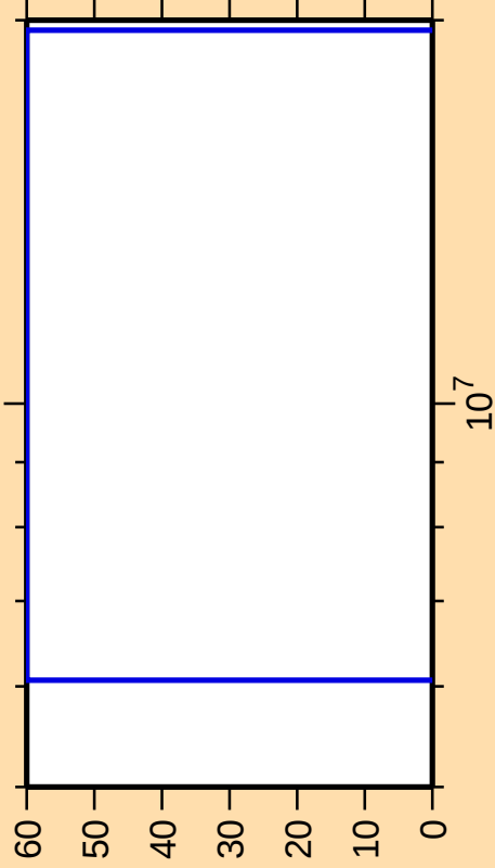
\Delta\sigma/\sigma vs. E for ^{149}\text{Sm}(n,d)
