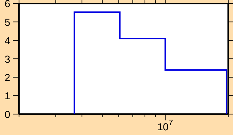
\Delta\sigma/\sigma vs. E for ^{149}\text{Sm}(n,\text{nonel.})
