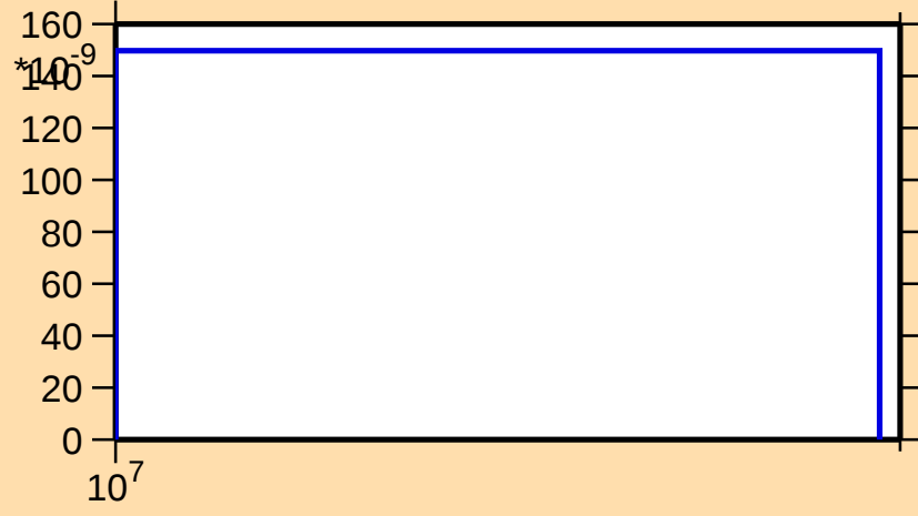
\sigma vs. E for ^{149}\text{Sm}(n,\text{nd})
