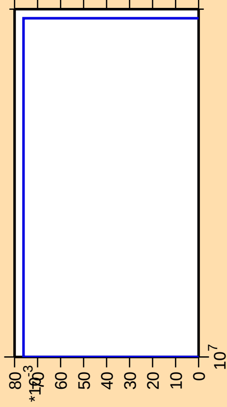
\Delta\sigma/\sigma vs. E for ^{149}\text{Sm}(n,3n\alpha)
