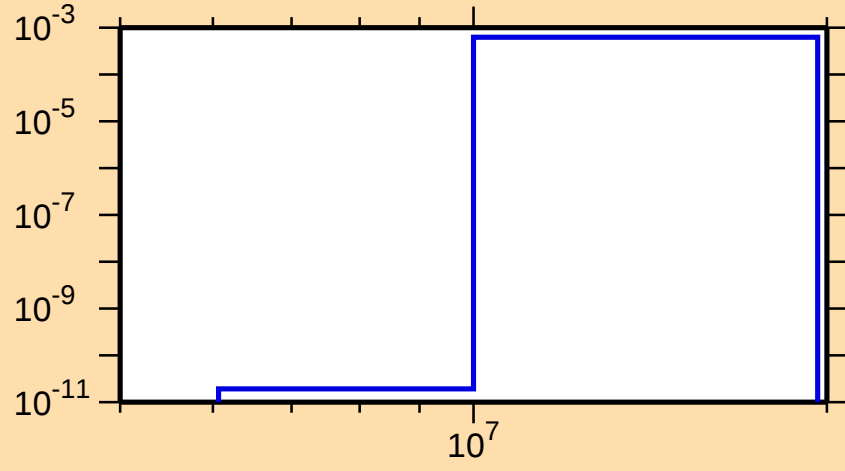
\sigma vs. E for ^{149}\text{Sm}(n,np)
