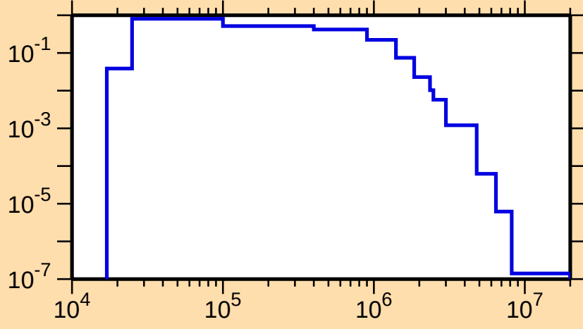
\sigma vs. E for ^{149}\text{Sm}(n,n_1)
