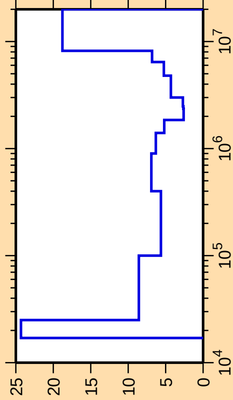
\Delta\sigma/\sigma vs. E for ^{149}\text{Sm}(n,\text{inel.})
