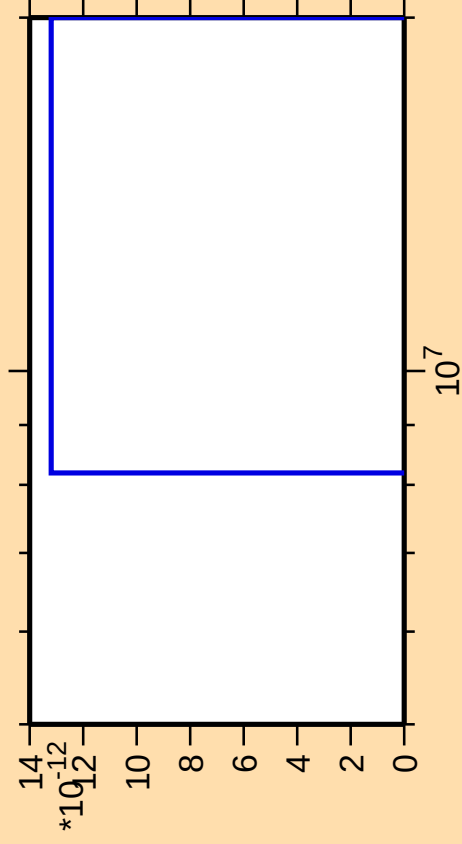
\Delta\sigma/\sigma vs. E for ^{149}\text{Sm}(\text{mt } 11)
