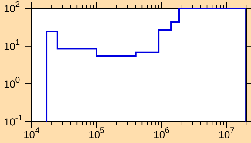
\Delta\sigma/\sigma vs. E for ^{149}\text{Sm}(n,n_1)
