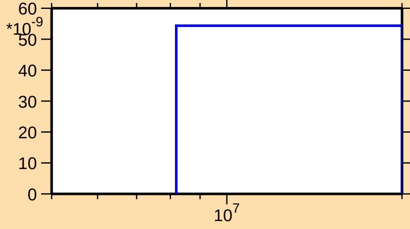
\sigma vs. E for ^{149}\text{Sm}(n,2np)
