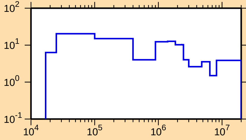
\Delta\sigma/\sigma vs. E for ^{149}\text{Sm}(n,\text{tot.})
