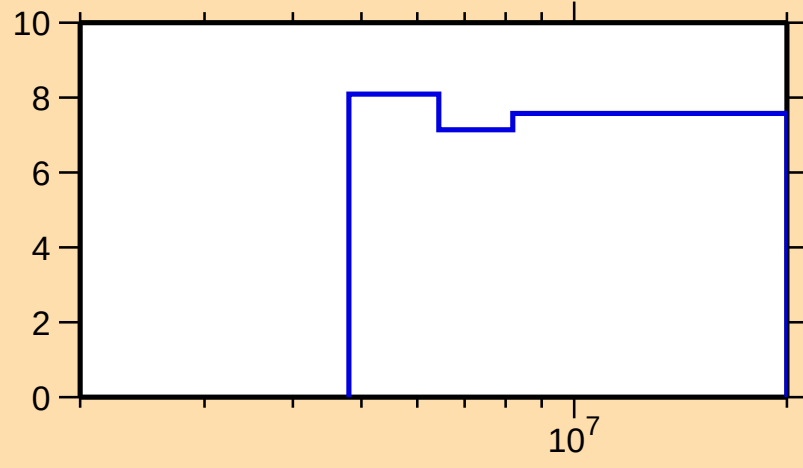
\Delta\sigma/\sigma vs. E for ^{149}\text{Sm}(n,2n)
