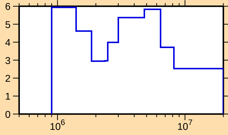
\Delta\sigma/\sigma vs. E for ^{149}\text{Sm}(n,\text{nonel.})
