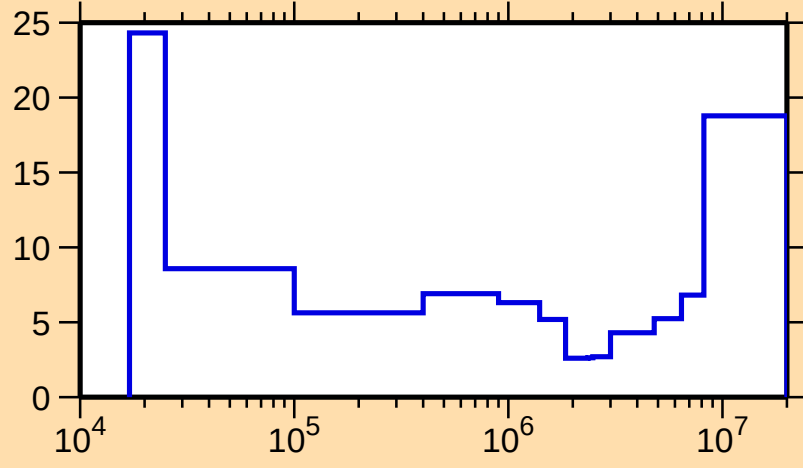
\Delta\sigma/\sigma vs. E for ^{149}\text{Sm}(n,\text{inel.})
