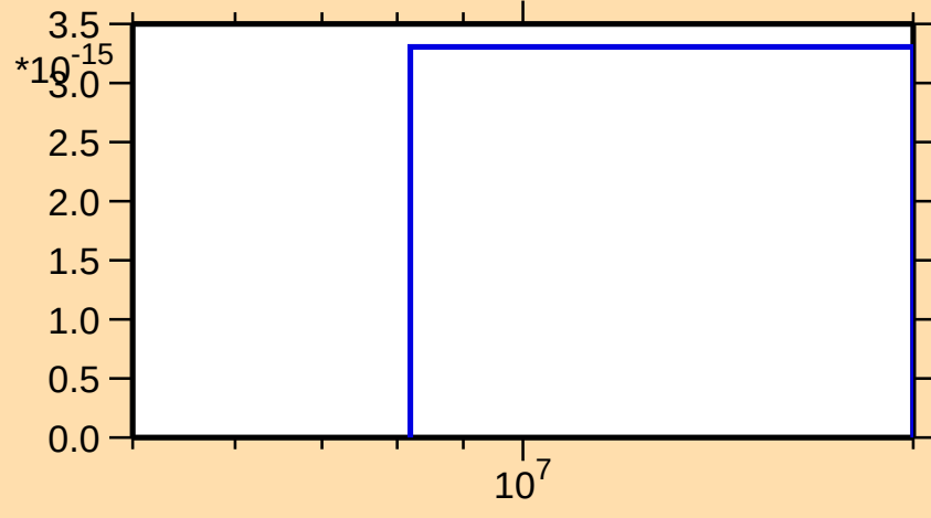
\sigma vs. E for ^{149}\text{Sm}(\text{mt } 34)
