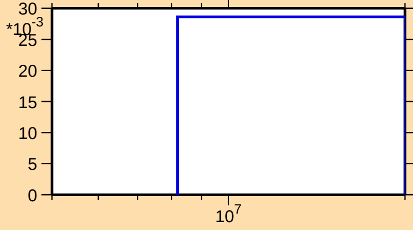
\sigma vs. E for ^{149}\text{Sm}(n,3n)
