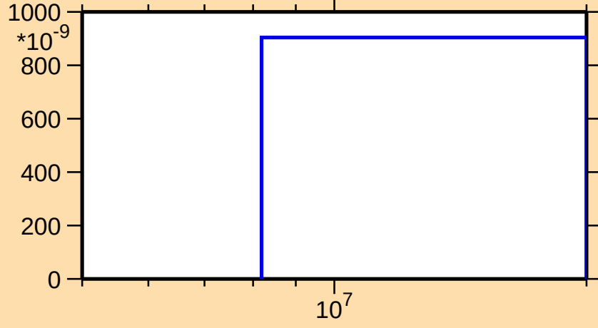
\sigma vs. E for ^{149}\text{Sm}(n,2n\alpha)
