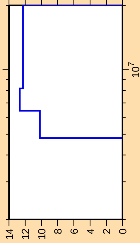
\Delta\sigma/\sigma vs. E for ^{149}\text{Sm}(n,n\text{cont.})
