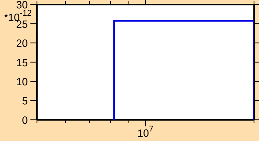
\sigma vs. E for ^{149}\text{Sm}(n,p\alpha)
