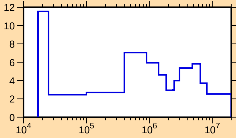
\Delta\sigma/\sigma vs. E for ^{149}\text{Sm}(n,\text{nonel.})
