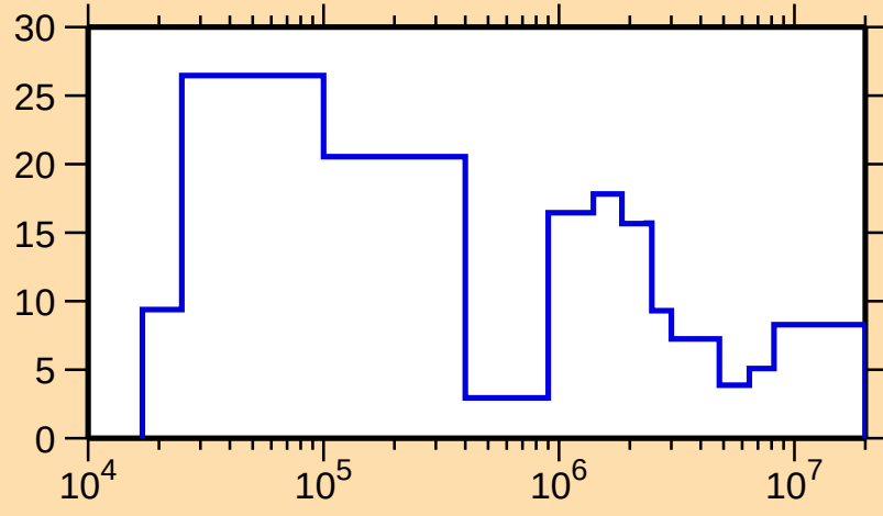
\Delta\sigma/\sigma vs. E for ^{149}\text{Sm}(n,\text{el.})
