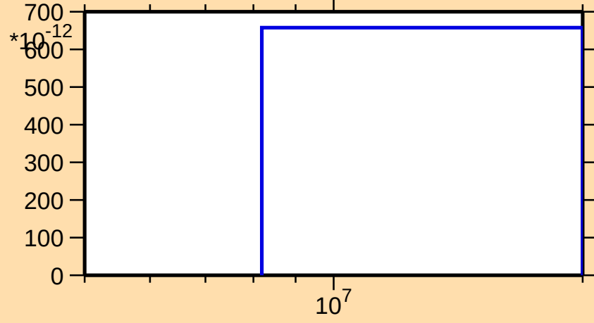
\sigma vs. E for ^{149}\text{Sm}(n,\text{He}3)
