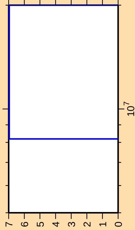
\Delta\sigma/\sigma vs. E for ^{149}\text{Sm}(n,3n)
