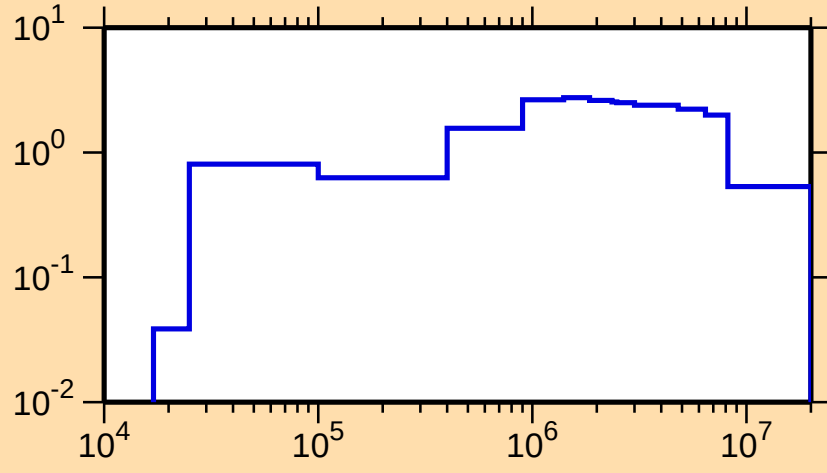
\sigma vs. E for ^{149}\text{Sm}(n,\text{inel.})
