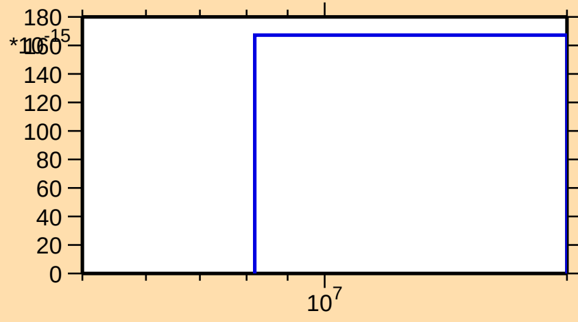
\sigma vs. E for ^{149}\text{Sm}(n,3n\alpha)
