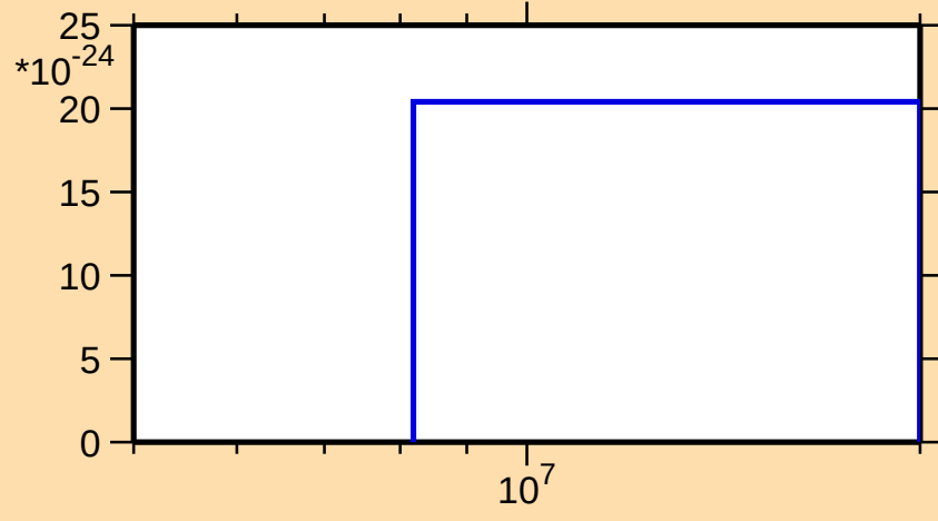
\sigma vs. E for ^{149}\text{Sm}(\text{mt } 11)
