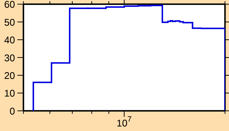
\Delta\sigma/\sigma vs. E for ^{151}\text{Sm}(n,\text{inel.})
