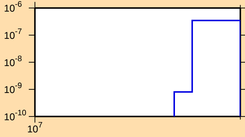
\sigma vs. E for ^{151}\text{Sm}(n,\text{nt})
