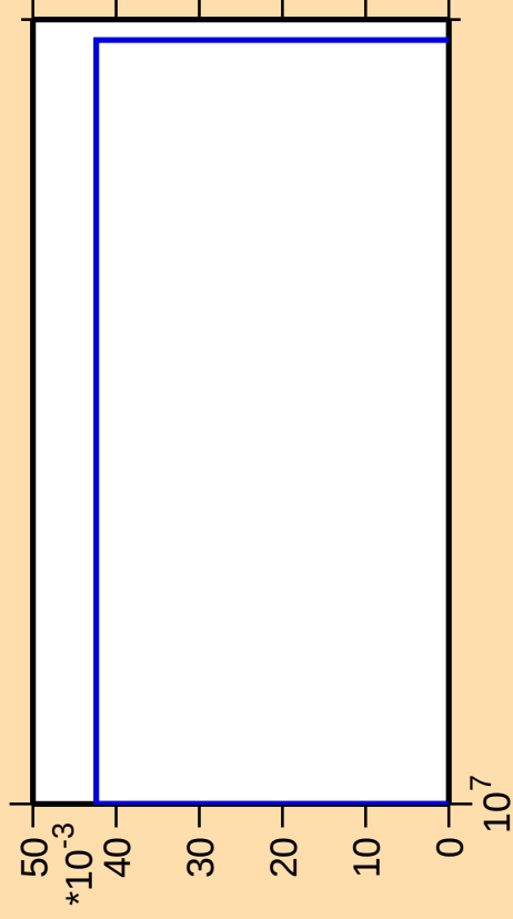
\Delta\sigma/\sigma vs. E for ^{151}\text{Sm}(n,3n\alpha)
