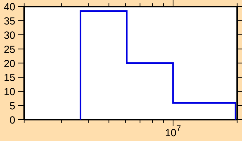
\Delta\sigma/\sigma vs. E for ^{151}\text{Sm}(n,2n)
