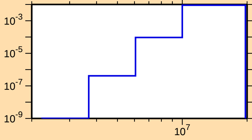
\sigma vs. E for ^{151}\text{Sm}(n,p)
