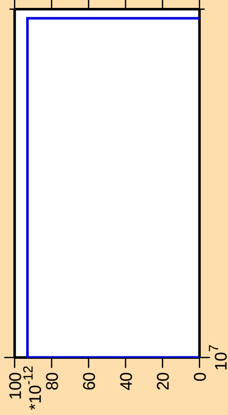
\Delta\sigma/\sigma vs. E for ^{151}\text{Sm}(\text{mt } 11)
