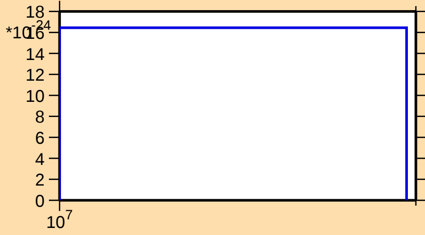
\sigma vs. E for ^{151}\text{Sm}(\text{mt } 11)
