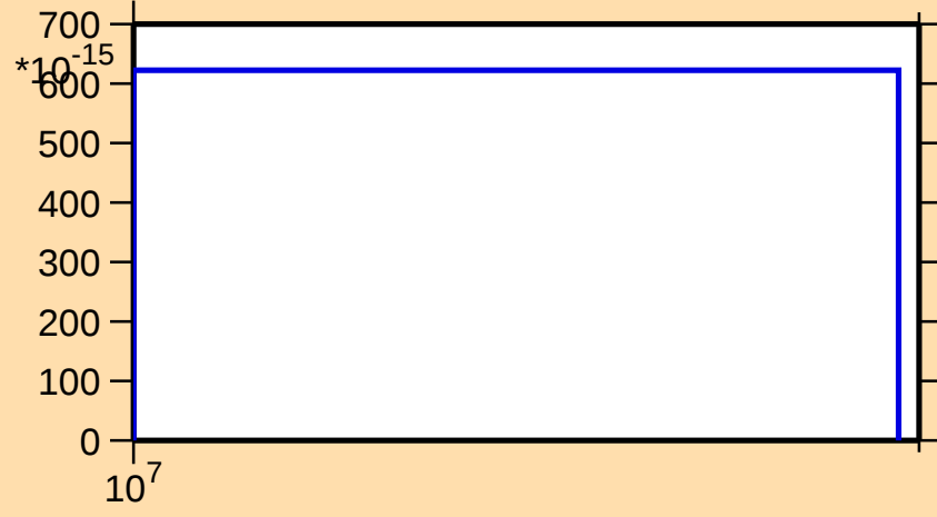
\sigma vs. E for ^{151}\text{Sm}(n,p\alpha)
