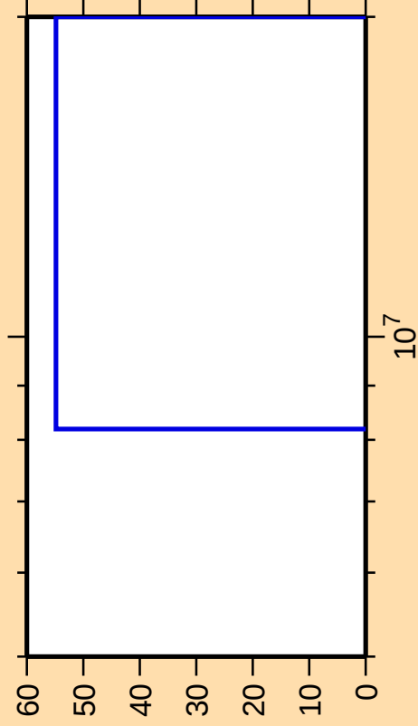
\Delta\sigma/\sigma vs. E for ^{151}\text{Sm}(n,np)
