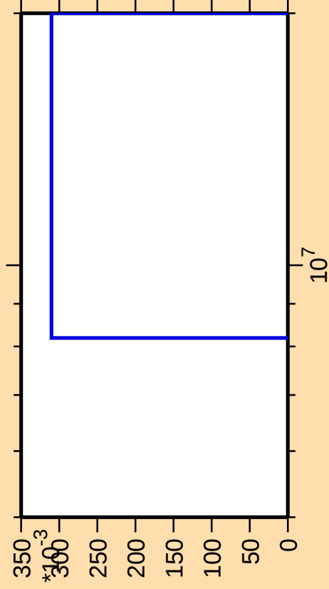
\Delta\sigma/\sigma vs. E for ^{151}\text{Sm}(n,p\alpha)
