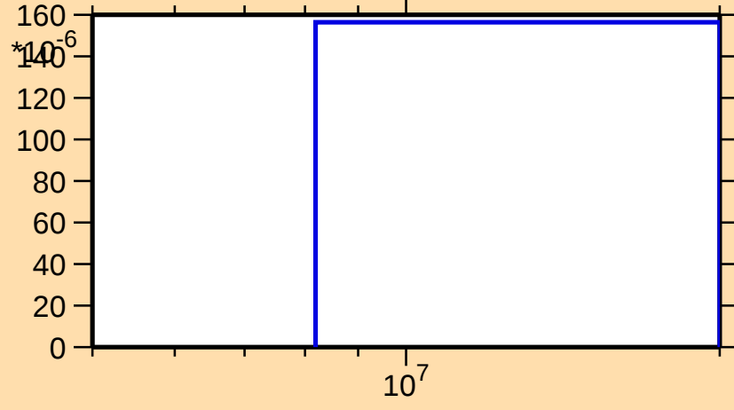
\sigma vs. E for ^{151}\text{Sm}(n,np)
