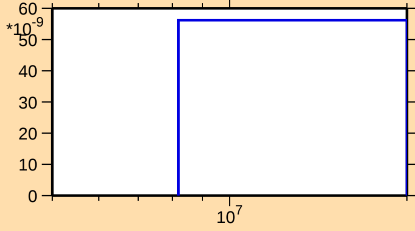
\sigma vs. E for ^{151}\text{Sm}(n,\text{nd})
