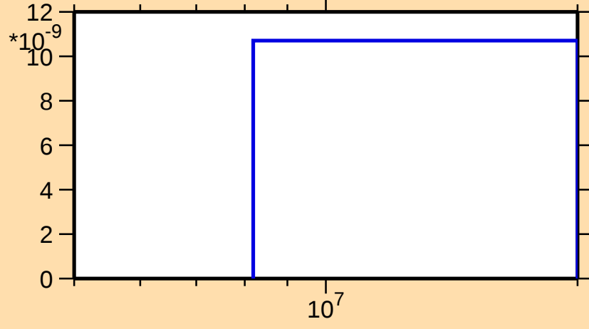
\sigma vs. E for ^{151}\text{Sm}(n,2np)
