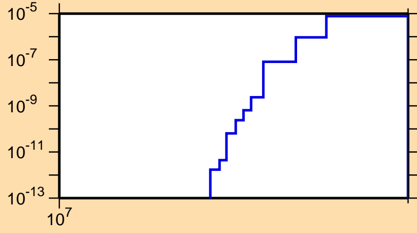
\sigma vs. E for ^{103}\text{Sn}(n,nd)
