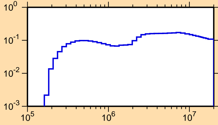
\sigma vs. E for ^{103}\text{Sn}(n,\text{inel.})
