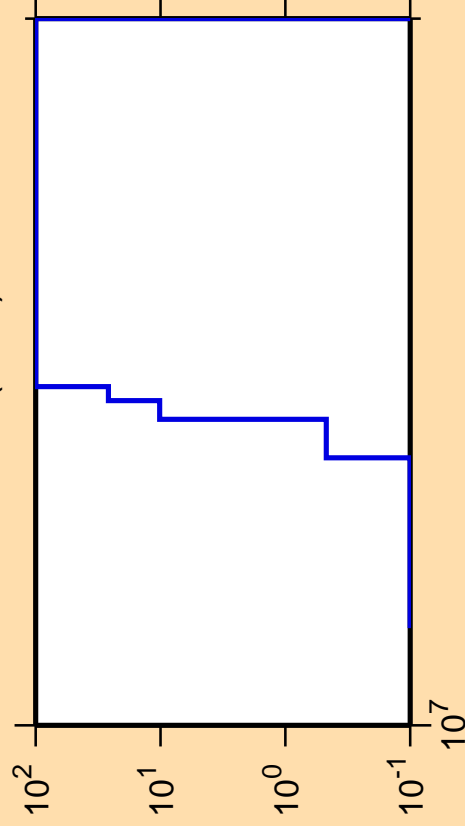
\Delta\sigma/\sigma vs. E for ^{103}\text{Sn}(n,nd)
