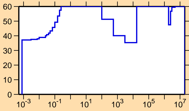
\Delta\sigma/\sigma vs. E for ^{103}\text{Sn}(n,\gamma)
