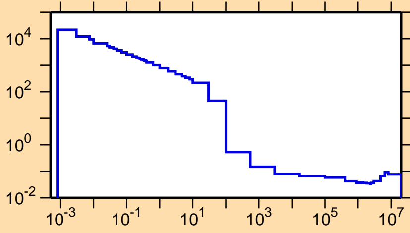
\sigma vs. E for ^{103}\text{Sn}(n,\alpha)
