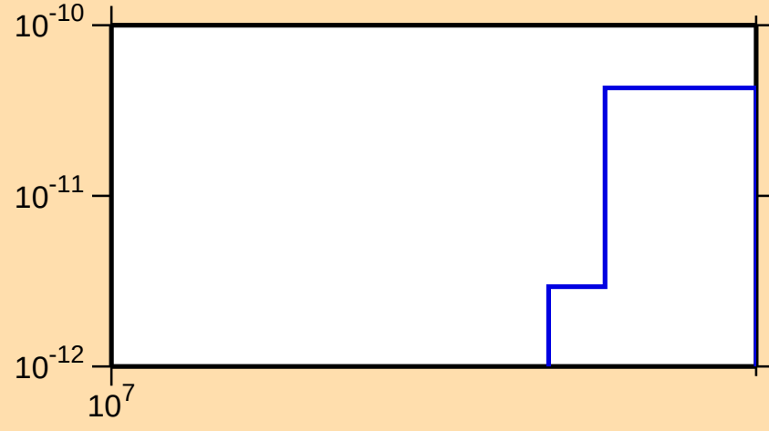
\sigma vs. E for ^{117}\text{Sn}(n,p\alpha)
