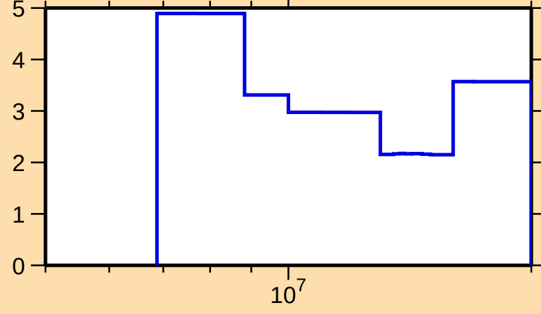
\Delta\sigma/\sigma vs. E for ^{117}\text{Sn}(n,\text{el.})
