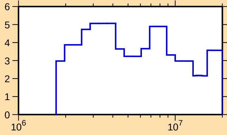
\Delta\sigma/\sigma vs. E for ^{117}\text{Sn}(n,\text{el.})
