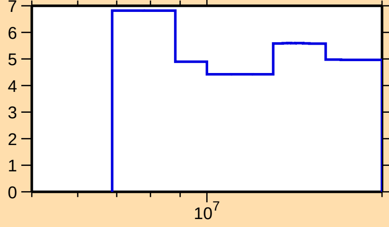
\Delta\sigma/\sigma vs. E for ^{117}\text{Sn}(n,\text{nonel.})
