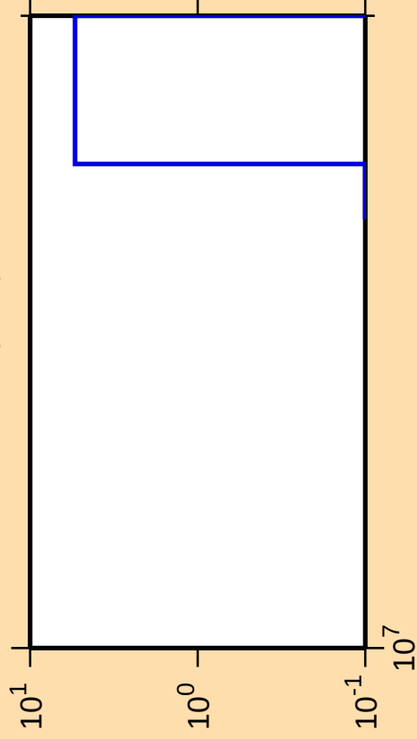
\Delta\sigma/\sigma vs. E for ^{117}\text{Sn}(n,nt)
