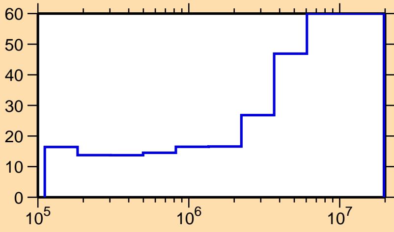
\Delta\sigma/\sigma vs. E for ^{117}\text{Sn}(n,n_1)
