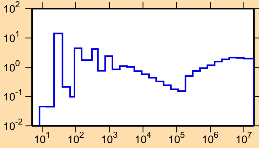
\sigma vs. E for ^{117}\text{Sn}(n,\text{nonel.})
