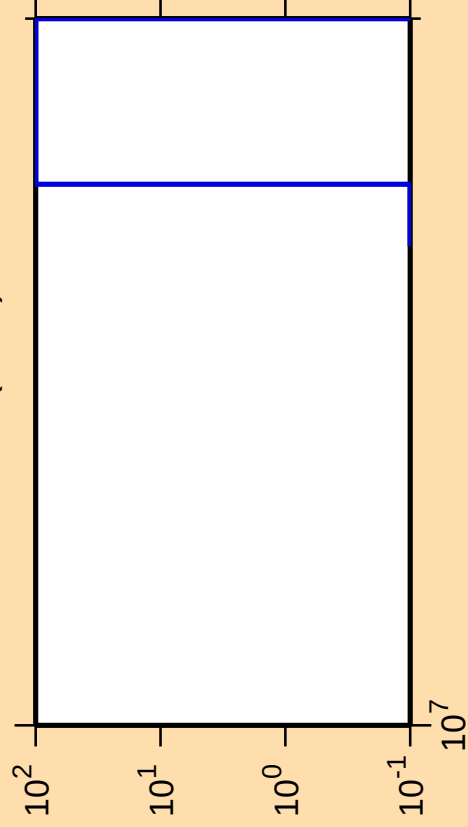
\Delta\sigma/\sigma vs. E for ^{118}\text{Sn}(n,\text{nd})
