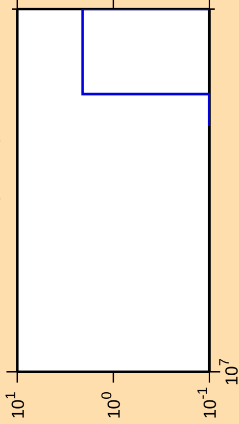
\Delta\sigma/\sigma vs. E for ^{118}\text{Sn}(n,2n\alpha)
