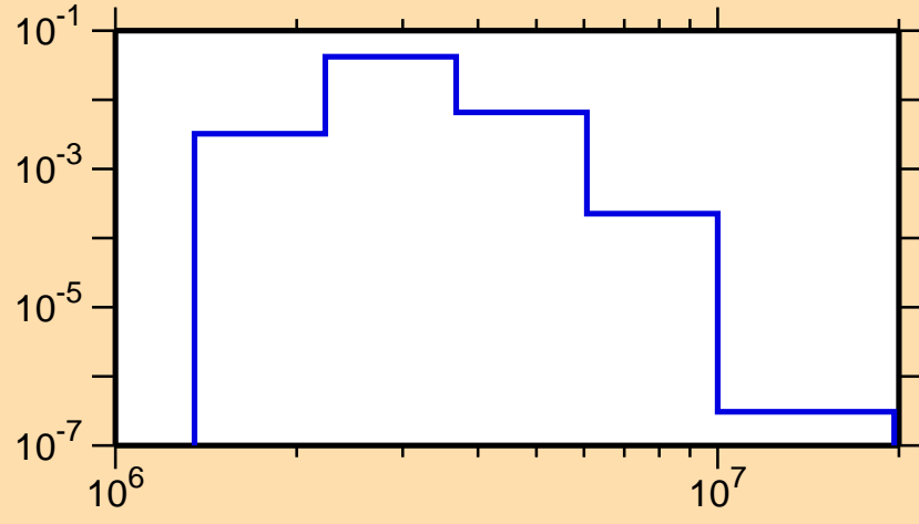
\sigma vs. E for ^{118}\text{Sn}(n,n_4)
