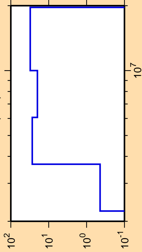
\Delta\sigma/\sigma vs. E for ^{118}\text{Sn}(n,\alpha)
