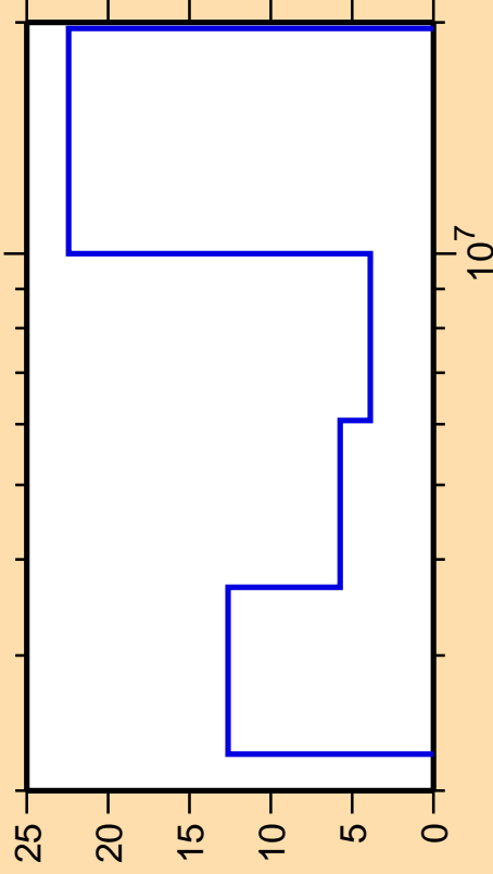
\Delta\sigma/\sigma vs. E for ^{118}\text{Sn}(n,n_{\text{cont}}) .
