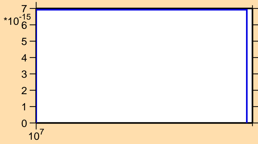
\sigma vs. E for ^{118}\text{Sn}(n,2n\alpha)
