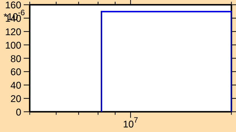
\sigma vs. E for ^{118}\text{Sn}(n,3n)
