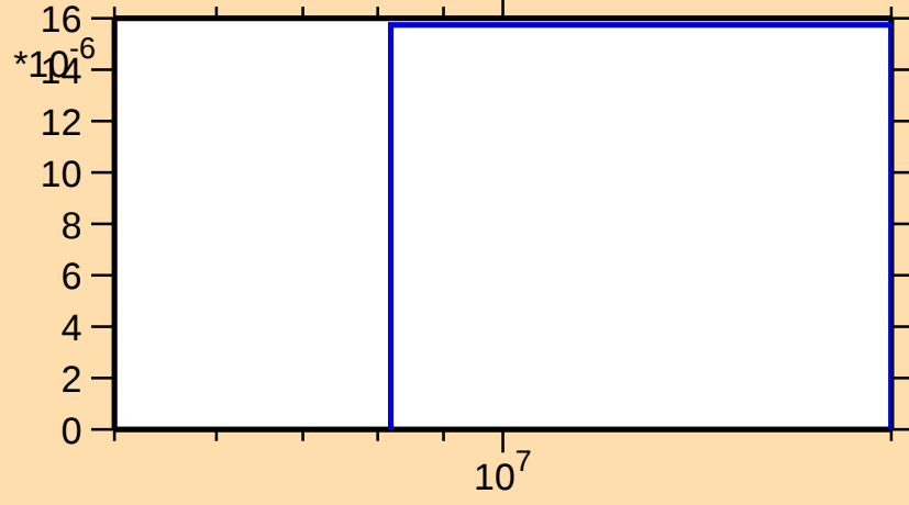
\sigma vs. E for ^{118}\text{Sn}(n,n\alpha)
