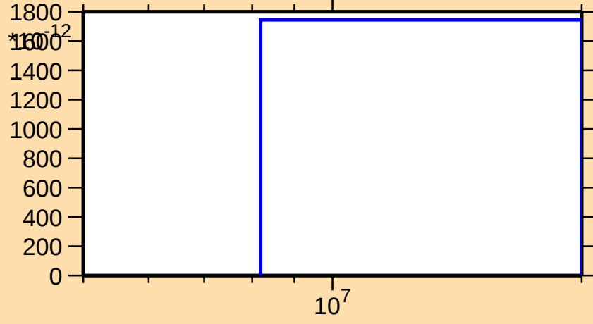
\sigma vs. E for ^{119}\text{Sn}(n,\text{nd})
