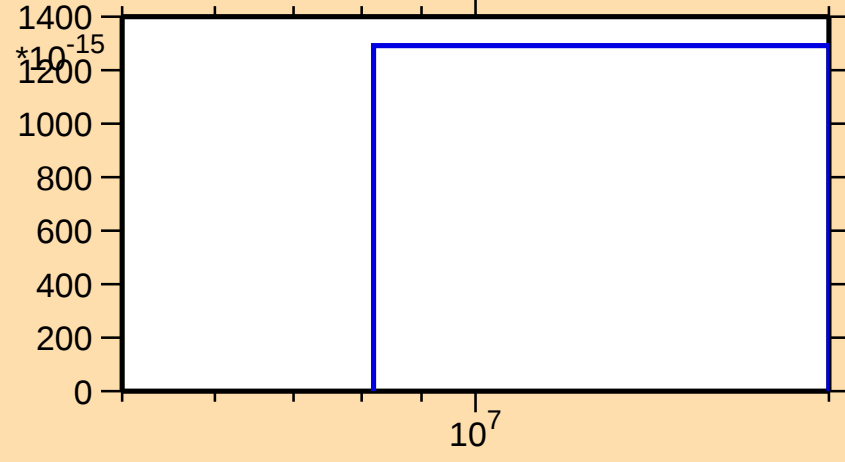
\sigma vs. E for ^{119}\text{Sn}(n,\text{He}3)
