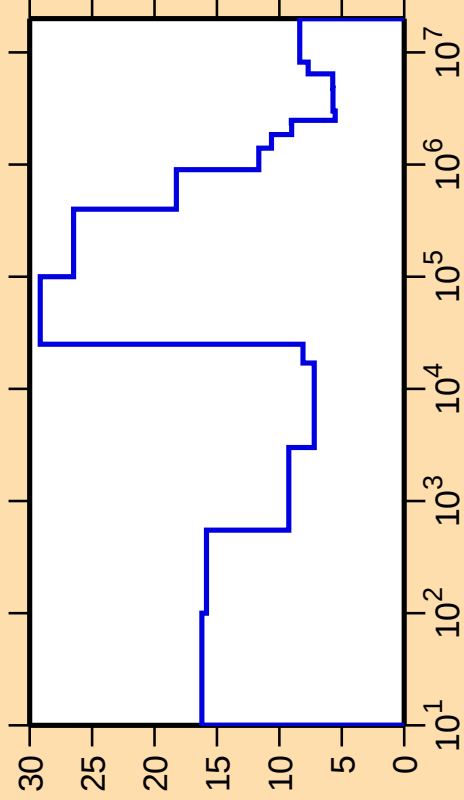
\Delta\sigma/\sigma vs. E for ^{119}\text{Sn}(n,\text{nonel.})
