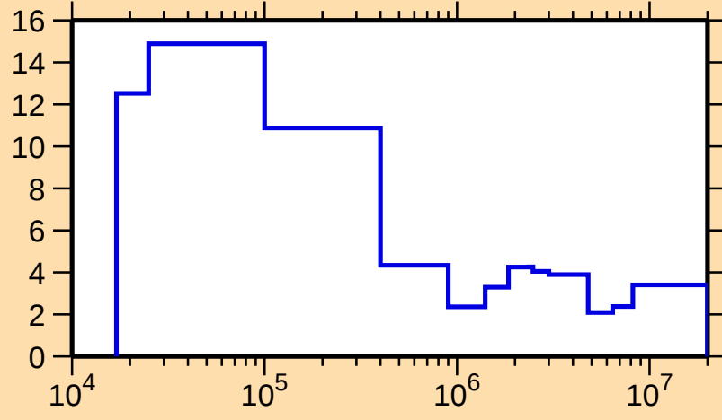
\Delta\sigma/\sigma vs. E for ^{119}\text{Sn}(n,\text{tot.})
