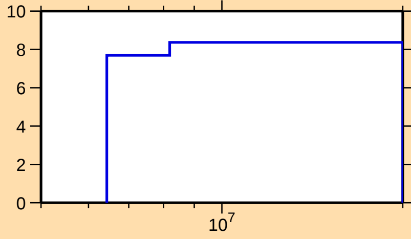
\Delta\sigma/\sigma vs. E for ^{119}\text{Sn}(n,\text{nonel.})
