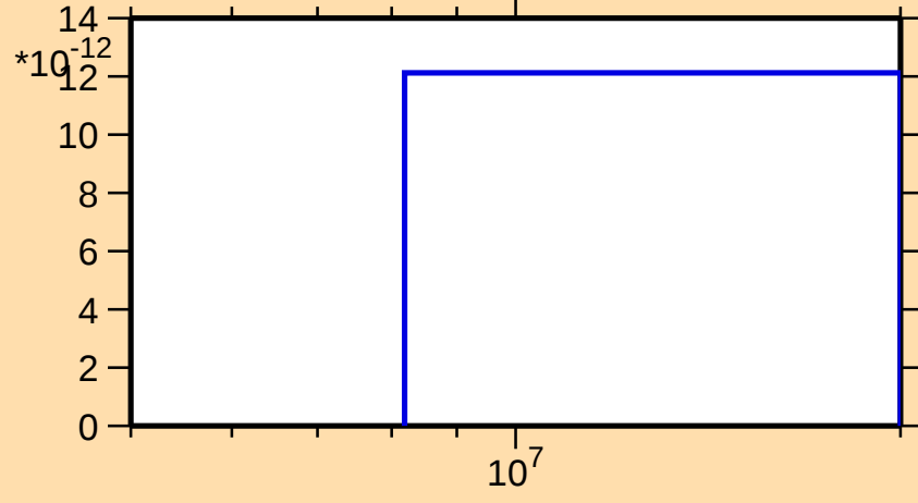
\sigma vs. E for ^{119}\text{Sn}(n,2n\alpha)
