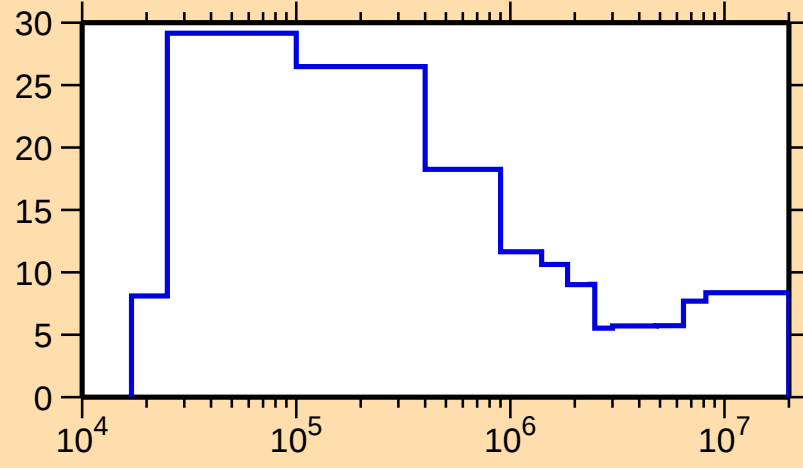
\Delta\sigma/\sigma vs. E for ^{119}\text{Sn}(n,\text{nonel.})
