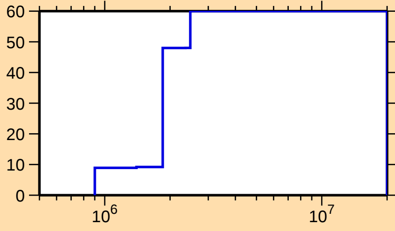
\Delta\sigma/\sigma vs. E for ^{119}\text{Sn}(n,n_1)
