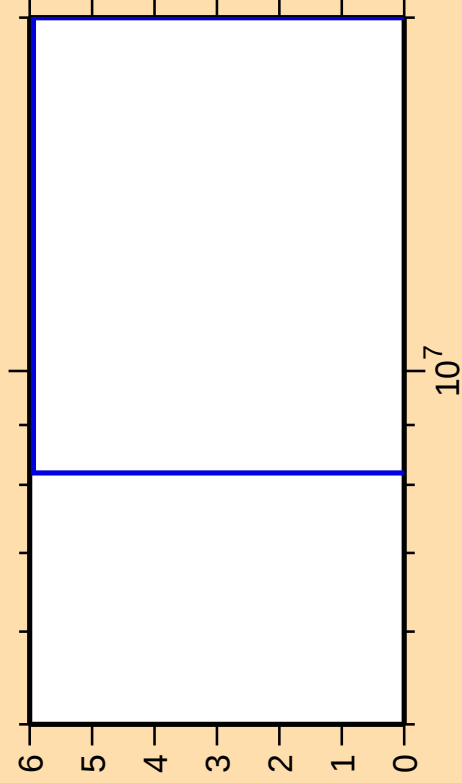
\Delta\sigma/\sigma vs. E for ^{119}\text{Sn}(n,2n\alpha)
