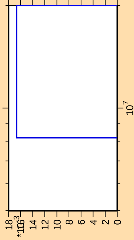
\Delta\sigma/\sigma vs. E for ^{119}\text{Sn}(n,nt)
