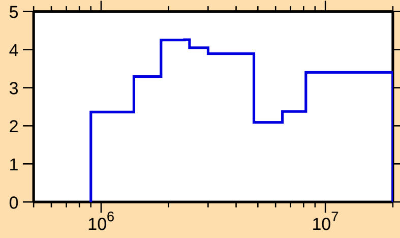
\Delta\sigma/\sigma vs. E for ^{119}\text{Sn}(n,\text{tot.})
