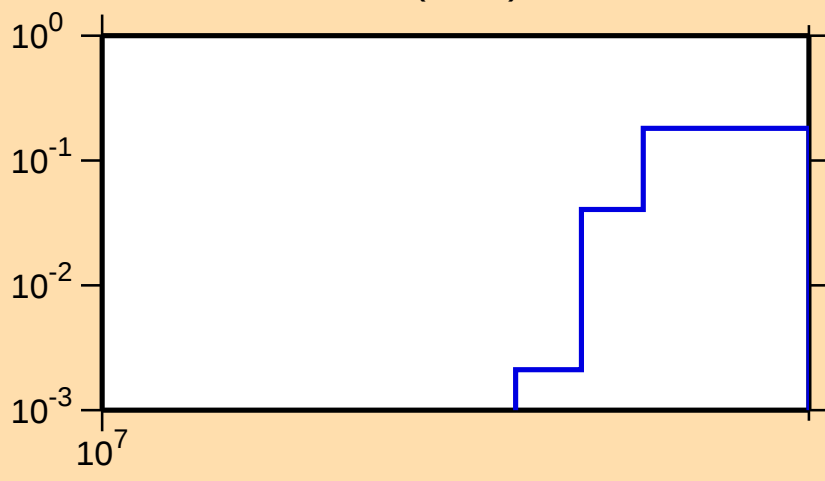
\sigma vs. E for ^{121}\text{Sn}(n,3n)
