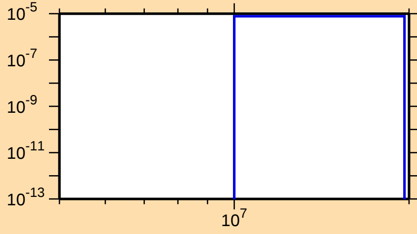
\sigma vs. E for ^{121}\text{Sn}(n,n\alpha)
