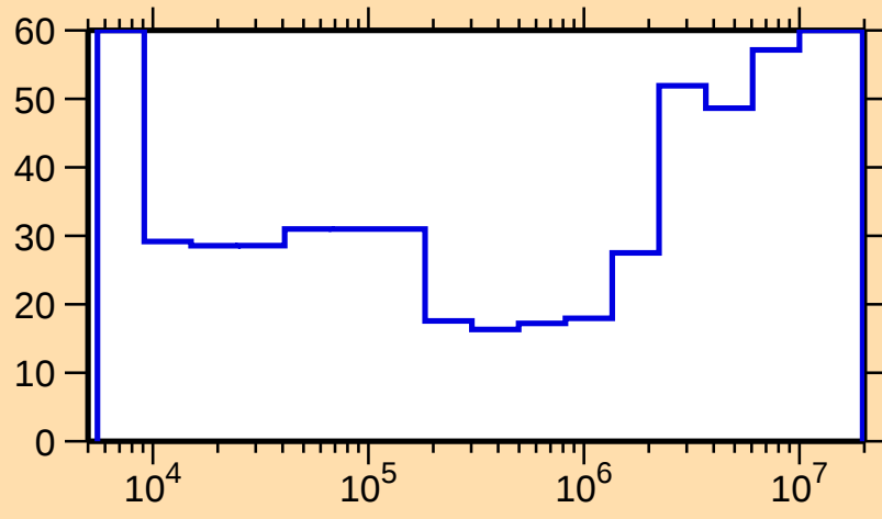
\Delta\sigma/\sigma vs. E for ^{121}\text{Sn}(n,n_1)
