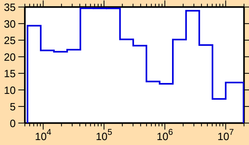
\Delta\sigma/\sigma vs. E for ^{121}\text{Sn}(n,\text{el.})
