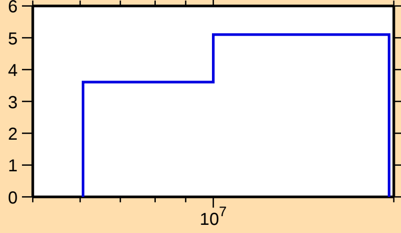
\Delta\sigma/\sigma vs. E for ^{121}\text{Sn}(n,\text{tot.})
