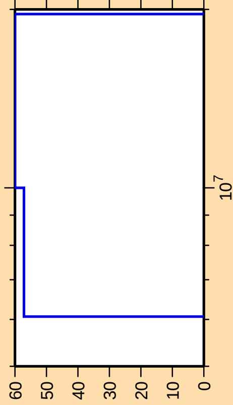
\Delta\sigma/\sigma vs. E for ^{121}\text{Sn}(n,n_1)
