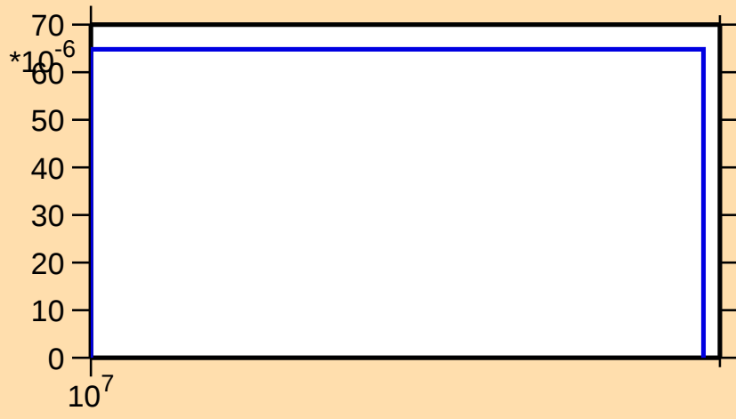
\sigma vs. E for ^{121}\text{Sn}(n,np)
