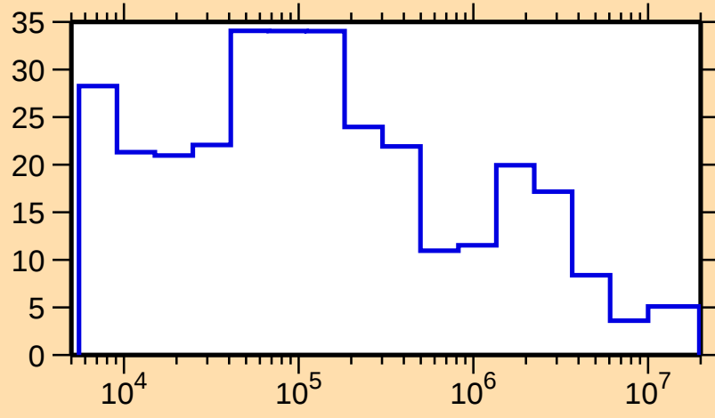
\Delta\sigma/\sigma vs. E for ^{121}\text{Sn}(n,\text{tot.})
