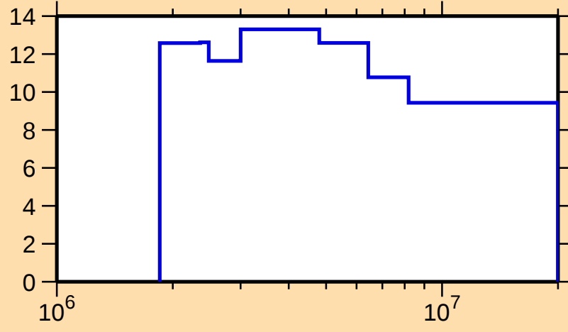
\Delta\sigma/\sigma vs. E for ^{121}\text{Sn}(n,\text{nonel.})
