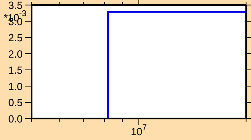
\sigma vs. E for ^{121}\text{Sn}(n,3n)
