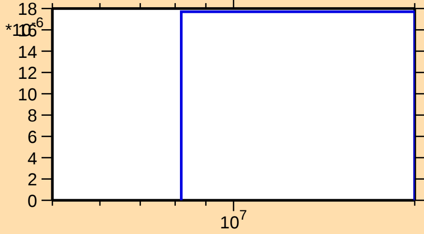
\sigma vs. E for ^{121}\text{Sn}(n,t)
