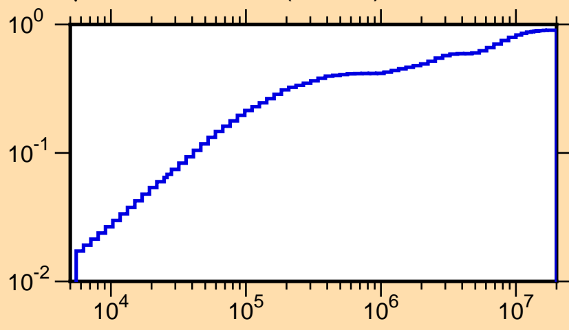
\mu vs. E for ^{124}\text{Sn}(\text{mt251})
