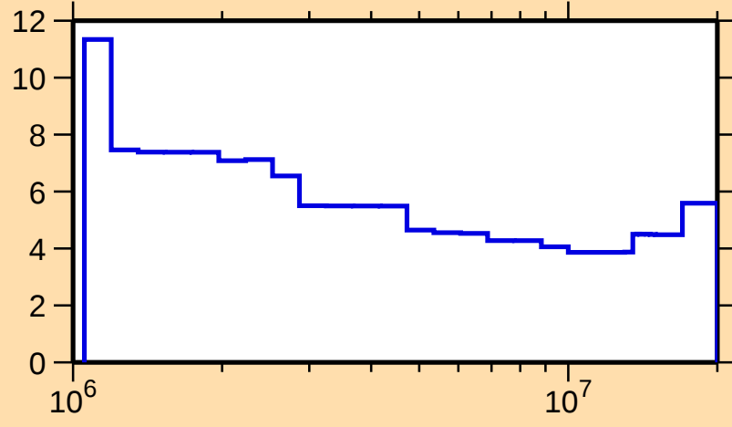
\Delta\sigma/\sigma vs. E for ^{124}\text{Sn}(n,\text{nonel.})
