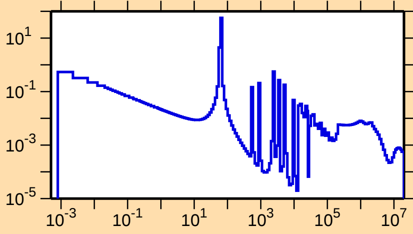
\sigma vs. E for ^{124}\text{Sn}(n,\gamma)
