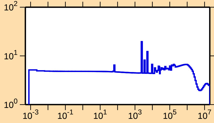
\sigma vs. E for ^{124}\text{Sn}(n,\text{el.})
